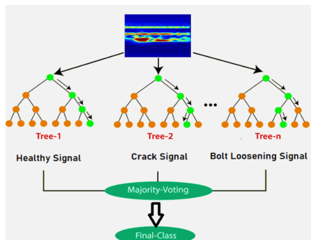
Fig. 5 Random Forest categorization structure
