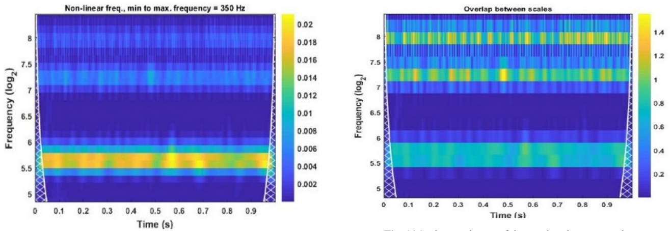
Fig. 12 Scalogram image of the non-linear frequency signal
