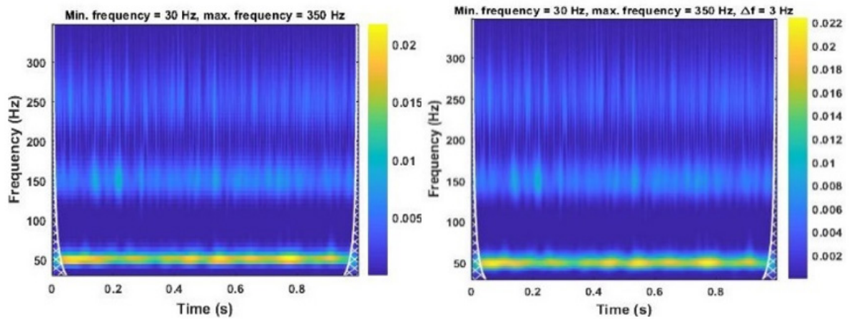
Fig. 11 Scalogram of linear frequency signal
