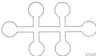
Fig. 2. The bridge-shaped sample, furnished with large areas for making low-ohmic contacts. large areas at the ends have the task to provide low-ohmic contacts. Furthermore, when making these contacts a heat treatment is often necessary which in this case can be done without heating that part of the sample which is under measurement.
