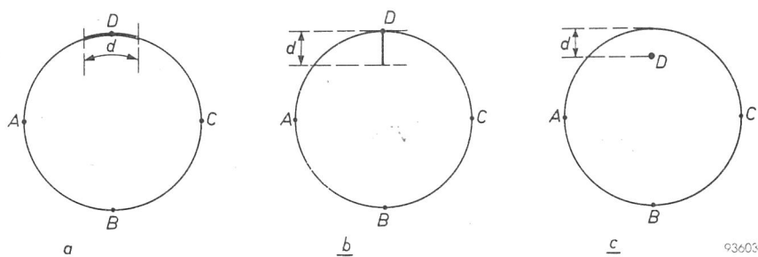
Fig. 8. Some special cases for which the error in the measurement of \varrho and \mu_H due to the finite length or the finite distance to the circumference of one contact has been calculated.
