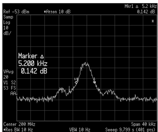
Fig. 4. Delayed self-heterodyne signal recorded by an spectral analyzer. Linewidth at -20 dB was measured to be 5.2 kHz.
