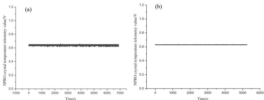
Fig. 7. The telemetry value of NPRO crystal temperature: (a) in-orbit and (b) on the ground test.
