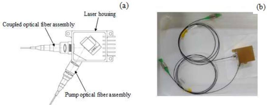
Fig. 3. (a) Schematic of NPRO laser and (b) Photograph of NPRO laser.
