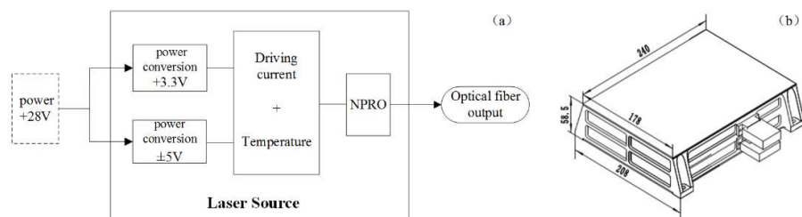
Fig. 1. (a) Schematic diagram of Laser source and (b) structure of Laser source.
