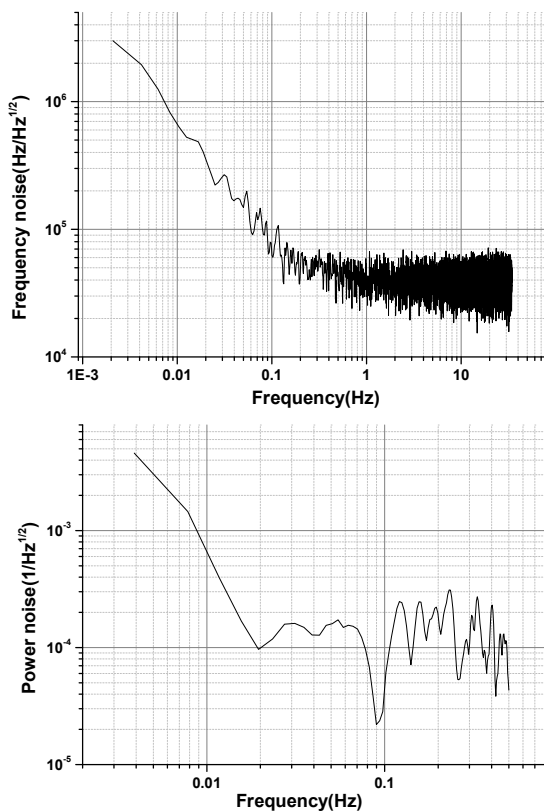
Fig. 5. Frequency and power noise spectral density of Laser source.
