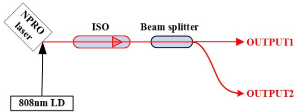
Fig. 2. Working principle diagram of Laser source.
