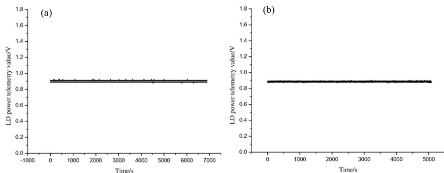
Fig. 6. The telemetry value of LD power: (a) in-orbit and (b) on the ground test.
