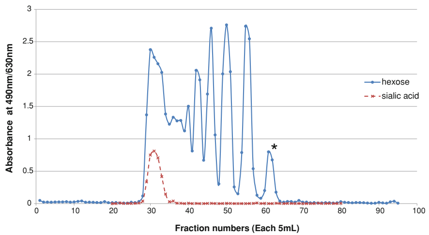
Fig. 1.4 Gel chromatogram of the carbohydrate fraction from tammar wallaby milk on BioGel P-2. The peak marked with * corresponds to lactose. Each fraction was monitored by the phenol- \text{H}_2\text{SO}_4 method at 490 nm for hexose and the periodate-resorcinol method at 630 nm for sialic acid
