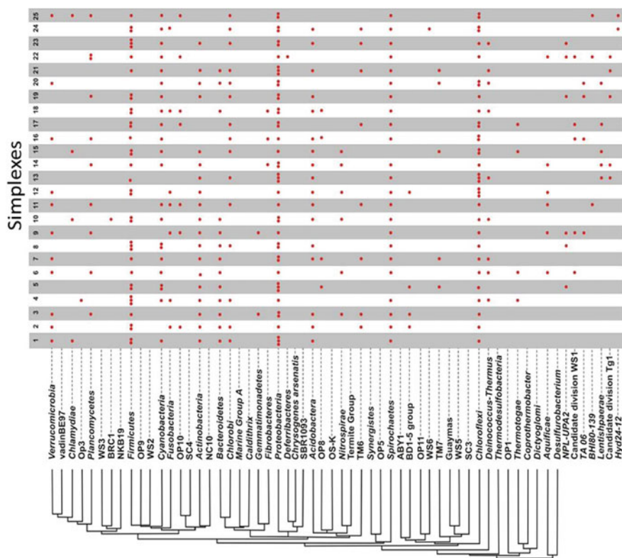
Fig. 16.2 Simplexes found in SILVA database distance matrix and taxonomic assignment (phylum) of their vertices
