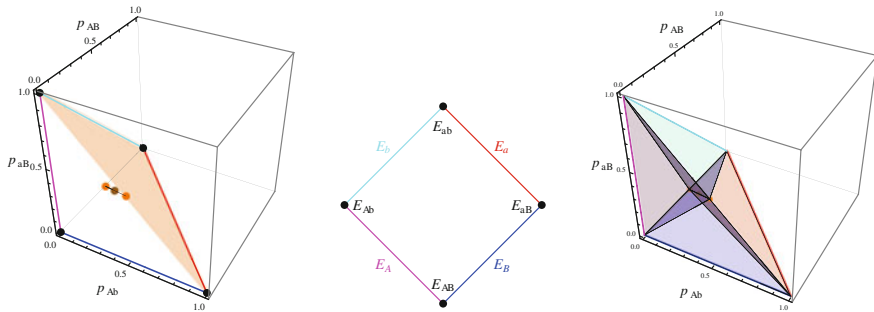
Fig. 17.2 Left three-dimensional phase space displaying the four families of equilibrium solutions: E_A ( p_{aB} axis, purple), E_B ( p_{AB} axis, blue), E_a (diagonal on the p_{Ab} - p_{AB} plane, red) and E_b (diagonal on the p_{aB} - p_{AB} plane, cyan); E_{ab} , E_{Ab} , E_{aB} and E_{AB} (vertices connecting the first family, black circles); EU_1 and EU_2 (midpoints of edges of the phase space not containing the first family, orange circles); and ES (center, brown circle). The shaded light brown surface represents the top face of the tetrahedral phase space of equation p_{AB} + p_{Ab} + p_{aB} = 1 . Middle Schematic representation of the stable fixed points. Right Division of the phase space displaying the basins of attraction of type 1 fixed points
