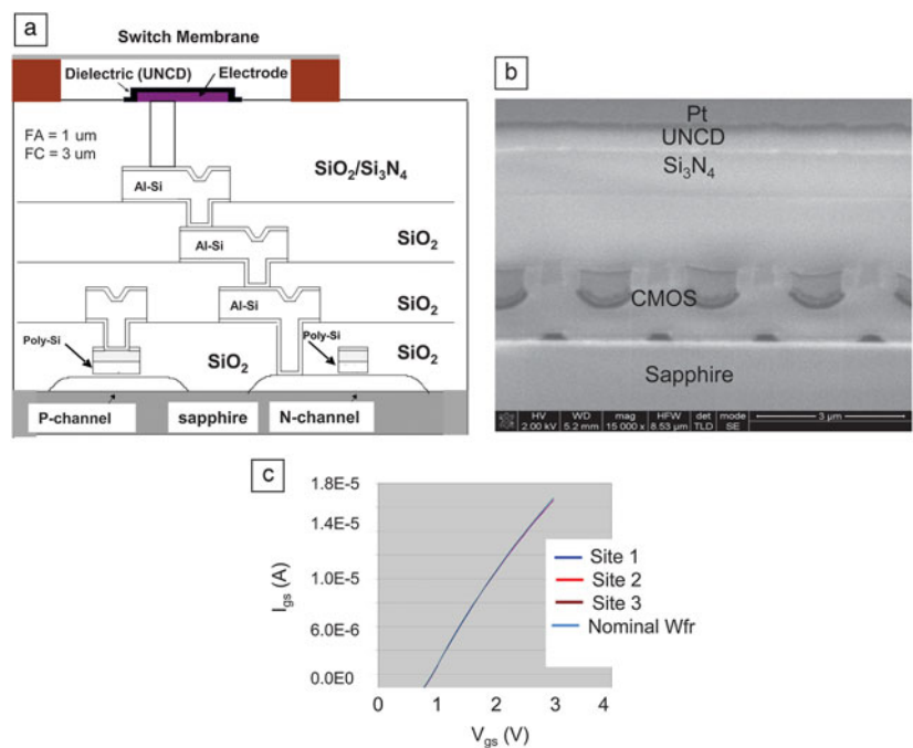
Figure 3. (a) Simplified schematic depicting integration of radio frequency microelectromechanical system switches with complementary metal oxide semiconductor (CMOS) on sapphire; (b) SEM image of a cross-section of ultrananocrystalline diamond (UNCD) film on CMOS on sapphire, produced by focused ion beam-induced etching; and (c) corresponding electrical performance of the integrated UNCD film/CMOS devices (from three different sites) after UNCD deposition compared to normal (before UNCD deposition) behavior. Reprinted with permission from Reference 30. © 2010 SPIE.
