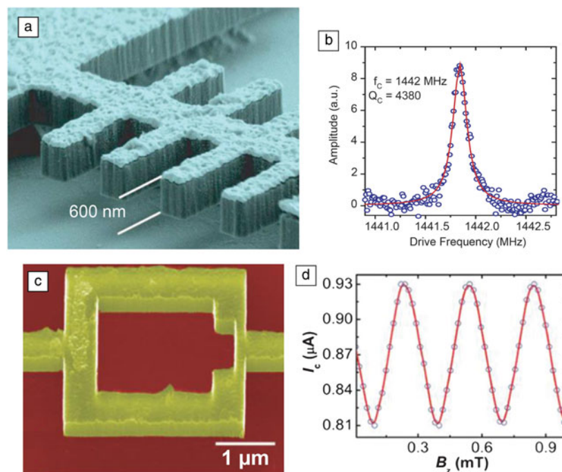
Figure 2. (a) Scanning electron micrograph of paddle cantilever structure. (b) Resonant frequency of paddle cantilever. (Reproduced with permission from Reference 18. © 2007 AIP Publishing.) (c) Diamond superconducting quantum interface device; the Josephson junctions in this device were created by making very narrow channels of diamond ( \sim 100 nm wide), which act as weak links. (d) Oscillations in the critical current as a function of magnetic field. Reproduced with permission from Reference 22. © 2011 American Chemical Society.
