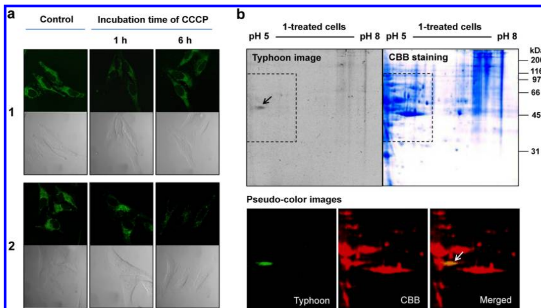
Figure 4. Analysis of probe 1 immobilized in mitochondria of HeLa cells. (a) The effect of CCCP, a recognized mitochondrial uncoupler, on the fluorescence confocal images of compounds 1 and 2 in HeLa cells. The lower images represent the corresponding bright field images. (b) 2D-gel of proteins collected from cells incubated with 1 for 5 h at 37 °C. The dotted lines define areas of Typhoon and CBB (coomassie brilliant blue) staining. These images were pseudocolored with green and red, respectively, and merged. Bands corresponding to fluorescent 1 -fixed proteins are shown with arrows. Typhoon images showing fluorescent bands were obtained using an excitation wavelength of 457 nm. All bands were visualized by CBB staining.
