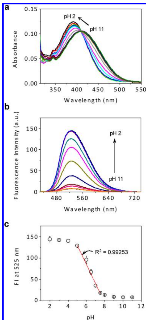
Figure 2. Changes in the optical features of 2 as a function of pH. Absorption (a) and fluorescence (b) spectra of 2 (10.0 and 1.0 \mu M, respectively) recorded at different pH values (2.0, 3.0, 4.0, 5.0, 6.0, 6.5, 7.0, 7.5, 8.0, 9.0, 10.0, 11.0). (c) Plot of fluorescence intensity (FI) at 525 nm vs pH. The dots are based on the average of three separate measurements with the error bars showing the standard deviation. All data were obtained using an excitation wavelength of 407 nm in 33 mM buffer solution containing 1% (v/v) DMSO at 37 ^{\circ} C.
