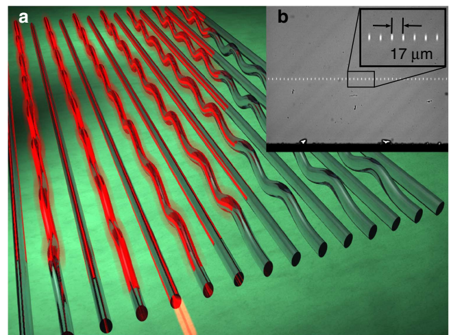
Figure 3 | Experimental realization of dissipative \mathcal{PT} -symmetric lattices.
