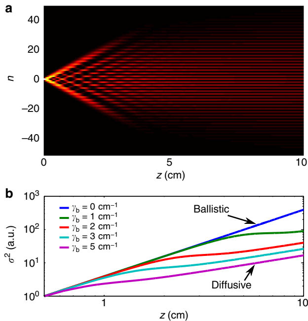
Figure 2 | Wave evolution in dissipative \mathcal{PT} -symmetric lattices.
