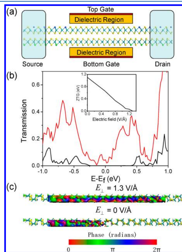
Figure 4. Dual-gated field effect transistor based on the A-A' MoS 2 bilayer conformation. (a) Schematic model. The channel is 4.9 nm long, and the electrodes are composed of doping homogeneous bilayer MoS 2 . Dark green ball, Mo; yellow ball, S; blue ball, N; light green ball, Cl. (b) Transmission spectrum under E_{\perp} = 0 V/Å (black line) and 1.3 V/Å (red line). Inset: ZTG as a function of the applied electric field. (c) Transmission eigenstates at E_f and at the (0,0) point of the k -space under E_{\perp} = 0 V/Å and 1.3 V/Å. The isovalue is 0.1 au.
