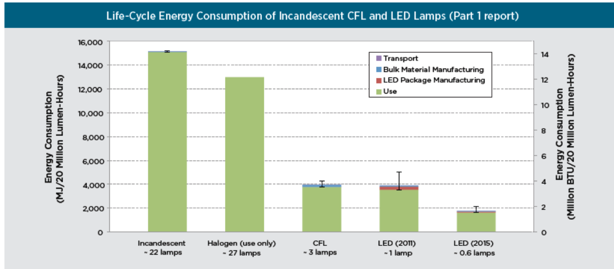
FIGURE 3.9 ENERGY CONSUMPTION COMPARISON FROM DOE LCA STUDY [54]
