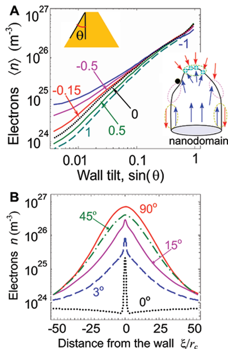
Figure 3. (A) Dependence of the carrier concentration \langle n(\xi) \rangle averaged across the wall thickness on the wall tilt, \sin \theta . Calculations were performed for the head-to-head 180^\circ walls and with different flexoelectric coupling coefficient f_{12} = (-1, -0.5, -0.15, 0, 0.5, 1) \times 10^{-10} \text{ m}^3/\text{C} (as labeled). Inserts show the definition of angle \theta and a schematic of a nanodomain exhibiting both straight (uncharged, yellow outline) c+/c- and curved (slightly charged, purple outline; strongly charged, green outline) domain walls, the associated directions of spontaneous polarization (blue and red arrows) and a defect (black). (B) Dependence of electron density for 180^\circ domain wall with different slope angles \theta = 90, 45, 15, 3 , and 0^\circ as a function of distance ( \xi/r_c ) perpendicular to the domain wall (correlation length r_c \approx 0.5 \text{ nm} ).
