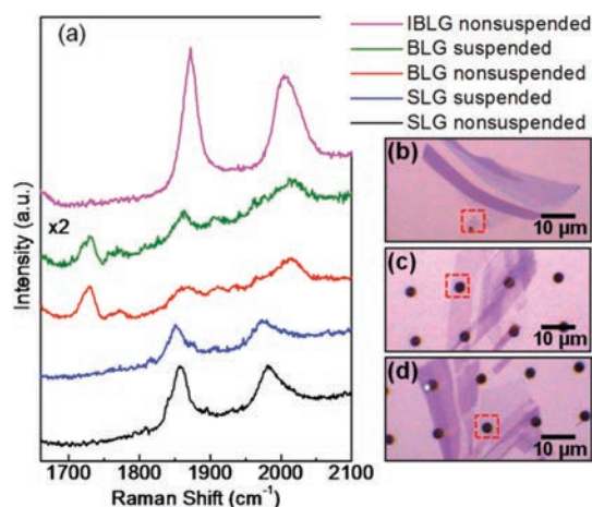
Figure 4. (a) Raman spectra of the suspended SLG and BLG, and the nonsuspended SLG, BLG, and the incommensurate BLG (IBLG). (b) Optical image of the incommensurate BLG on a 300 nm \text{SiO}_2/\text{Si} substrate. (c, d) Optical images of graphene sheets on a patterned 300 nm \text{SiO}_2/\text{Si} substrate covering holes. The incommensurate BLG, the suspended BLG, and the suspended SLG were marked by red dash-line square on panels b, c, and d, respectively.
