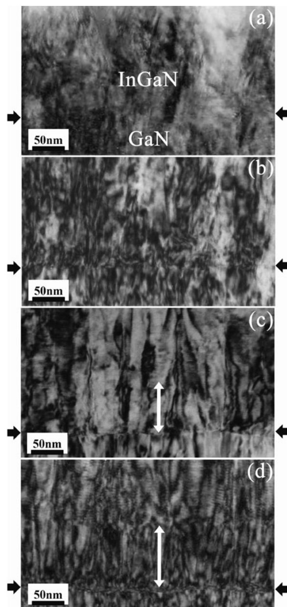
Figure 1. Bright-field transmission electron microscopy micrograph of the \text{In}_x\text{Ga}_{1-x}\text{N} layers with (a) 11%, (b) 33%, (c) 47%, and (d) 67% indium content. Horizontal black arrows indicate the positions of InGaN/GaN interface and white vertical arrows indicate the average height without modulation above the InGaN/GaN interface.
