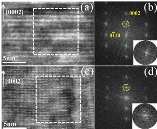
Figure 3. High-resolution transmission electron microscopy micrograph of the composition modulation within the \text{In}_{0.67}\text{Ga}_{0.33}\text{N} layer. a: Typical distribution of composition modulation on c -planes, and the corresponding fast Fourier transform (FFT) image in (b). The inset image in (b) is the magnified 0001 (encircled) spot. c: Some areas have composition modulations on the \{0\bar{1}14\} planes, and the corresponding FFT image is in (d). The inset image in (d) is the magnified 0001 (encircled) spot.
