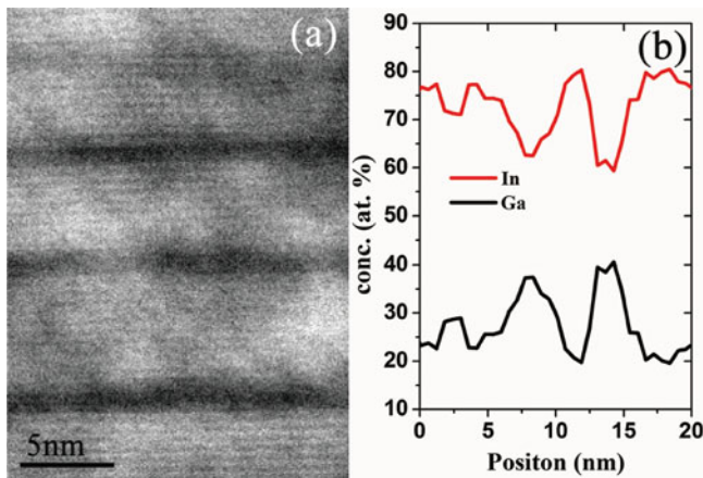
Figure 2. a: HAADF-STEM micrograph, and (b) EDS line spectra of the composition modulated region in the \text{In}_{0.67}\text{Ga}_{0.33}\text{N} sample. HAADF, high-angle annular dark-field; STEM, scanning transmission electron microscopy; EDS, energy-dispersive spectroscopy.
