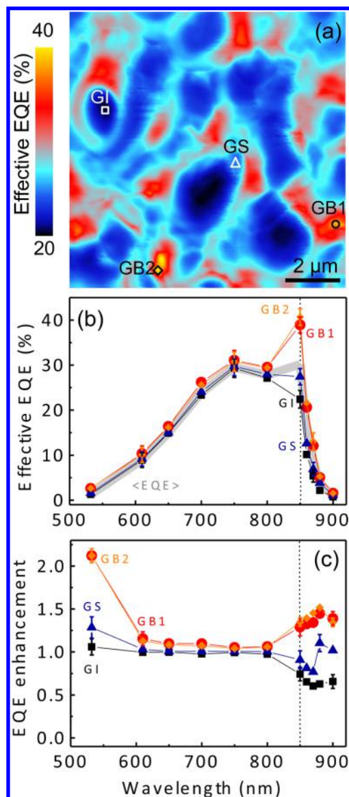
Figure 5. Mapping local variations in EQE with nanoscale resolution. (a) Effective EQE map for CdTe solar cell acquired using 850 nm wavelength as a local excitation source. (b) Effective EQE as a function of wavelength for selected regions of the CdTe layer. (c) EQE enhancement for the same region. GI, grain interior (black); GS, grain side (blue); GB, grain boundary (red, orange). The dashed line corresponds to the CdTe band gap. The error bars correspond to the standard deviation of three measurements, taken at each wavelength.
