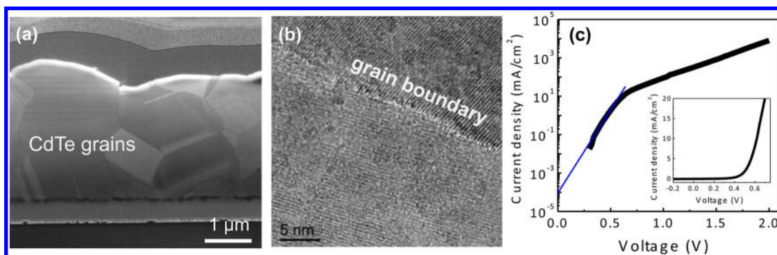
Figure 1. CdTe polycrystalline solar cells. (a) Cross-section SEM image of a thin-film CdTe solar cell showing micron-scale grains and interfaces with structural defects. (b) Atomic resolution TEM image showing a grain boundary (interface between two grains). (c) Semilog dark I – V curve. The blue line corresponds to the fit used to infer the shunt current. Inset: linear dark I – V showing diode behavior of CdTe/CdS solar cell device.
