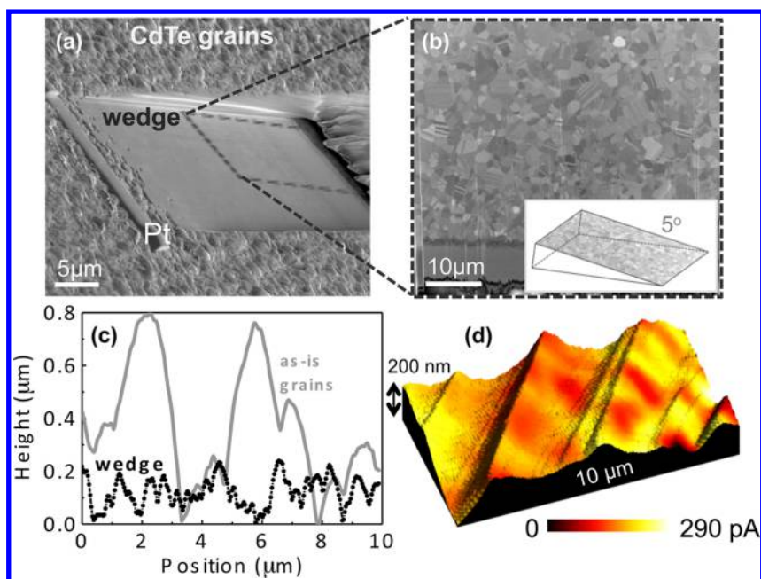
Figure 3. Analysis of topographic effects in nanoscale photocurrent scanning microscopy. (a,b) SEM images of wedge sculpted by Ga focused ion beam. Inset shows a schematic of the wedge shape. (c) Surface topography of CdTe grains before (as-is grains) and after (wedge) the milling process. (d) Three-dimensional topography overlaid with photocurrent measurement. Illumination source = 532 nm laser; incident power = 0.5 nW; NSOM probe = 200 nm. For the topography scan, set point = 0.95 V.
