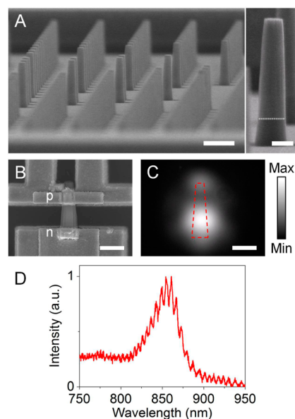
Figure 2. Fabrication and optical properties of a GaAs NW LED. (A) SEM image of vertical arrays of the NWs fabricated by EBL and dry etching. The scale bar is 2 \mu\text{m} . The right panel shows the magnified SEM image of a triangular cross-sectional single NW with a length of \sim 2.3 \mu\text{m} . The white dotted line indicates the sonication cleavage interface to separate NWs from the substrate. The scale bar is 500 nm. (B) SEM image of the fabricated NW LED. The scale bar is 1 \mu\text{m} . (C) EL image of the NW LED captured by a CCD camera. The NW in (B) was superimposed on the image as the red dotted line. The scale bar is 1 \mu\text{m} . (D) Measured EL spectrum from the NW LED. A current pulse with a peak value of 22.4 \mu\text{A} and a 10% duty cycle was injected.
