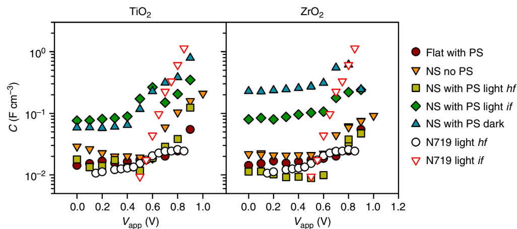
Fig. 5 | Capacitance analysis of \text{TiO}_2 and \text{ZrO}_2 and comparison with a solid DSSC using N719 dye. The left graph plots capacitance of the following: flat sample with PS; blank NS \text{TiO}_2 (0.35 \mu\text{m} thickness) with no PS; NS \text{TiO}_2 (0.55 \mu\text{m} thickness) with PS extracted from measurement under dark and under 1-sun illumination (light) conditions; and all-solid DSSC (2.2 \mu\text{m} thickness) with N719 as dye and spiro-MeOTAD as HTM. The right graph plots capacitance of the following: flat samples with PS; blank NS \text{ZrO}_2 (0.39 \mu\text{m} thickness) with no PS; NS \text{TiO}_2 (0.36 \mu\text{m} thickness) with PS extracted from measurements under dark and under 1-sun illumination (light) conditions; and all-solid DSSC (2.2 \mu\text{m} thickness) with N719 as dye and spiro-MeOTAD as the HTM. Capacitance has been normalized to the electrode volume. Capacitance for both graphs has been extracted by fitting the IS spectra from the if region if nothing else is indicated. In some cases, capacitance has been extracted from the hf region as it is indicated in the legend.
