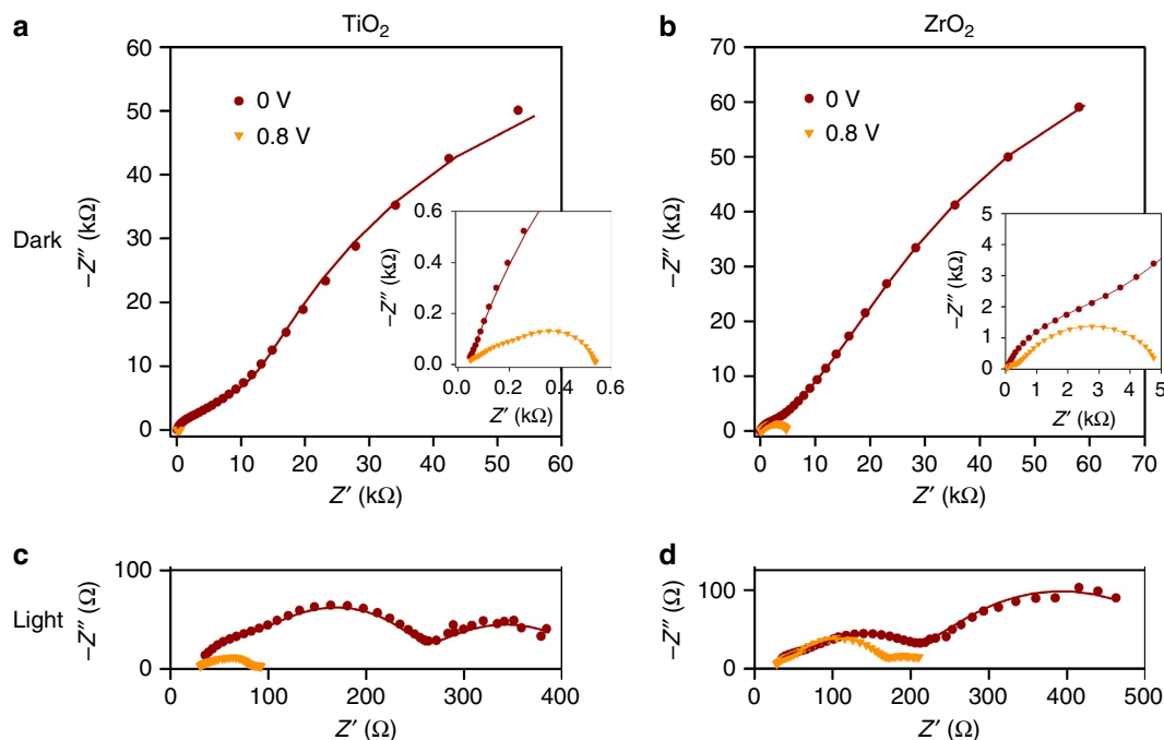
Figure 3 | Nyquist plots of lead iodine PS solar cells in \text{TiO}_2 and \text{ZrO}_2 electrodes. Nyquist plot of solar cells prepared as FTO/compact \text{TiO}_2 /nanostructured oxide/PS/spiro-MeOTAD/Au. The left column corresponds to the device using \text{TiO}_2 as the NS oxide, whereas the right column corresponds to the device with \text{ZrO}_2 , as shown in Fig. 1 and summarized in Table 1. (a) and (b) correspond to IS measurements under dark conditions; transmission line behaviour is clearly visible. The inset is a zoom of the low impedance region. (c) and (d) correspond to measurements under 1-sun illumination. Nyquist plots for two different applied DC signals, V_{\text{app}} , are shown in the graphs. Solid lines are the fits obtained using equivalent circuits previously used for solid DSSC with spiro-MeOTAD 22 and in some cases additional R-C feature to the TL for an accurate fitting, see Supplementary Fig. S9.
