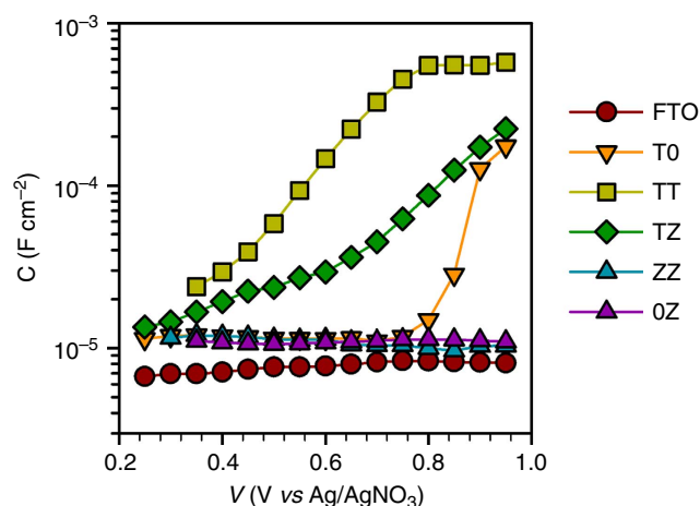
Figure 2 | Capacitance of non-sensitized electrodes. Capacitance has been extracted from IS measurements in liquid electrolyte with \text{I}^-/\text{I}_3^- redox couple. Capacitance of the bare conductive \text{SnO}_2/\text{F} (FTO) electrode is compared with electrodes with different layers of \text{TiO}_2 and \text{ZrO}_2 . The electrodes are called using the notation XY, where X is a compact layer, Y is a porous layer and T and Z are \text{TiO}_2 and \text{ZrO}_2 layers, respectively. O indicates no layer – that is, T0 compact \text{TiO}_2 layer with no nanoporous layer.
