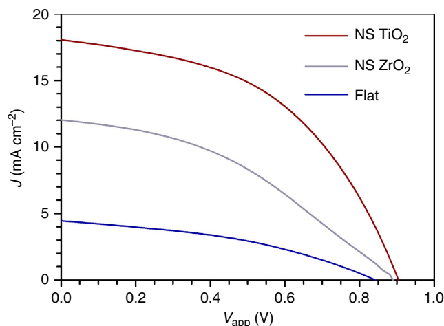
Figure 1 | Solar cell performance. Current–potential J – V curves of lead iodide PS with three different electrodes: FTO/compact TiO 2 (Flat), FTO/compact TiO 2 /nanostructured TiO 2 (NS TiO 2 ) and FTO/compact TiO 2 /nanostructured ZrO 2 (NS ZrO 2 ). Solar cell parameters and conversion efficiency are summarized in Table 1.
