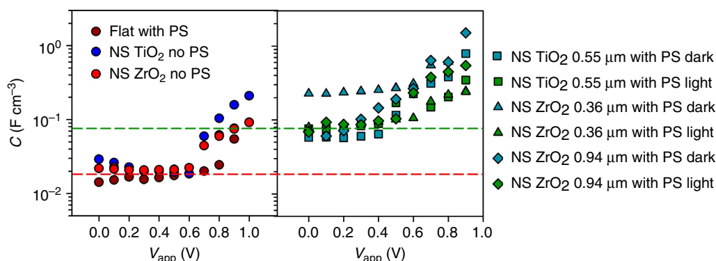
Fig. 4 | Capacitance analysis of flat samples and NS samples with and without PS. The left graph plots capacitance of flat with PS, and blank samples without PS, NS \text{TiO}_2 and \text{ZrO}_2 samples present NS layers of 0.35 \mu\text{m} \text{TiO}_2 and 0.39 \mu\text{m} \text{ZrO}_2 , respectively. The right graph plots the capacitance of NS \text{TiO}_2 and \text{ZrO}_2 samples with PS of samples with different NS layer thicknesses as indicated in the legend. Capacitance values obtained in measurements under dark and under 1-sun illumination (light) conditions are plotted. Capacitance for both graphs has been extracted by fitting the IS spectra from the if region as discussed in Supplementary Note 1. Capacitance has been normalized to the electrode volume. Red and green dashed lines are only eye guides to highlight the difference in capacitance obtained for samples with and without PS.
