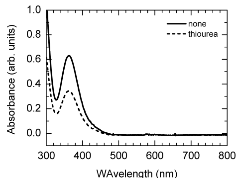
Figure 4. Absorption spectra of electrolyte (0.7 M MPIO and 0.05 M I 2 in acetonitrile) with and without thiourea as a function of wavelength.
