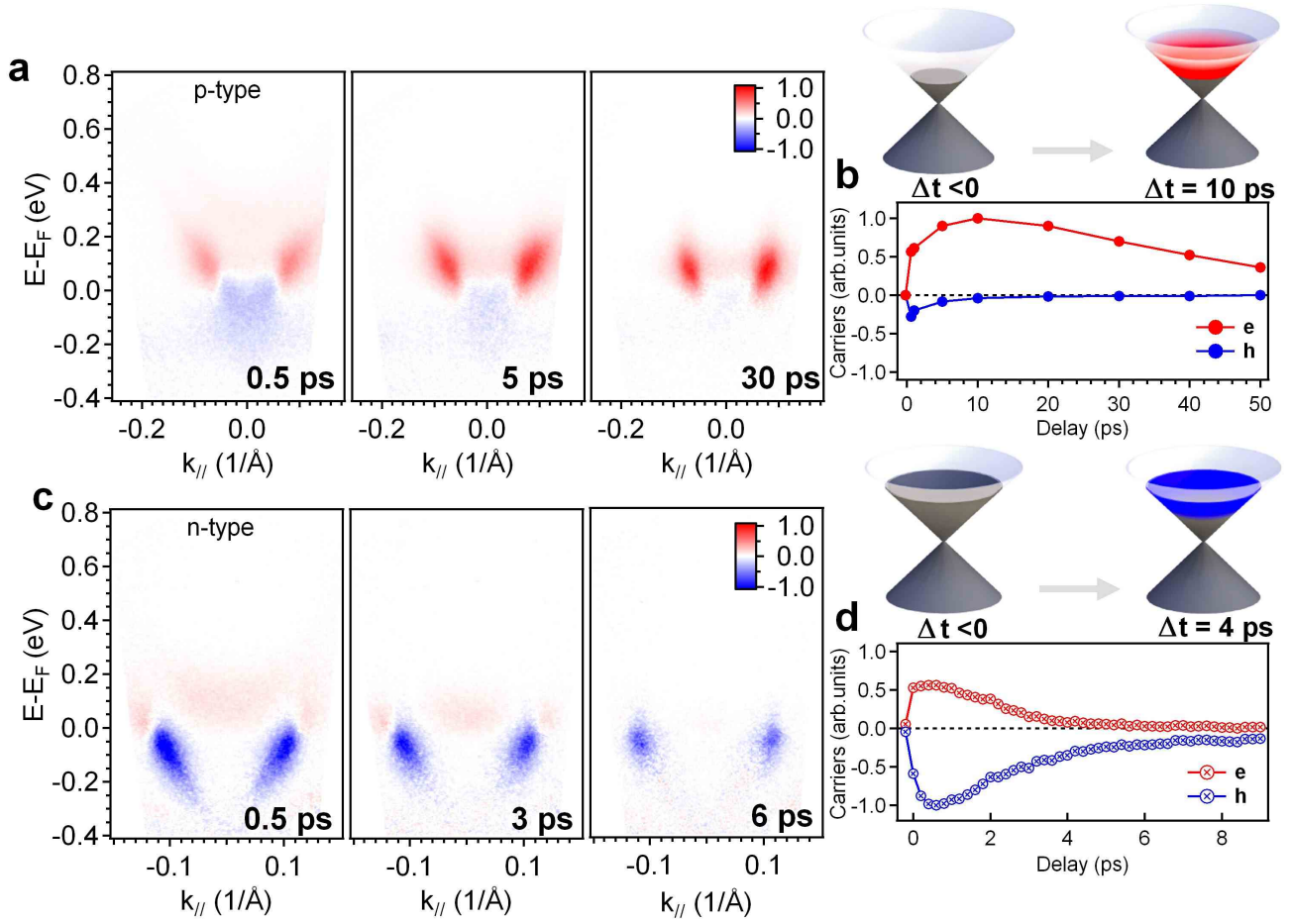
FIG. 3: Charge asymmetry of transient excess carriers. Excess electrons (red) and holes (blue) are detected from the difference of time-resolved ARPES images taken after and before photoexcitation. We present them in (a) for p-type \text{Bi}_{2.2}\text{Te}_3 and in (c) for n-type \text{Bi}_2\text{Te}_2\text{Se} . In (b) and (d) we present the time evolution of the detected excess carriers (electrons, e, and holes, h): a transient accumulation of holes is seen for the n-type specimen, and a much more pronounced asymmetry related to a strong and long lived accumulation of hot electrons in the Dirac cone for the p-type sample.
