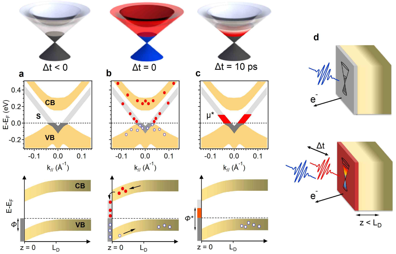
FIG. 5: Transient topological insulator state and non equilibrium surface 2D metallic layer in a nanoscale Schottky barrier. We compare \text{Bi}_{2.2}\text{Te}_3 (a) in its ground state, (b) right after photoexcitation and (c) in its photo-excited state for a delay \Delta t = 10 ps after optical pumping. For each case, the top panel represents a pictorial view of the Dirac cone with excess electrons (red) and holes (blue); the mid panel shows the schematic structure of the bands in reciprocal space and their filling at the surface ( z=0 ); and the bottom panel the corresponding band lineup in real space along the normal to the surface z . In (d) we present a schematic view of the experimental configuration: when the sample is in its ground state (top), ARPES probes the rest value \phi of the barrier between the chemical potential \mu and the top of the valence band; when the sample is photoexcited with a pump pulse, time resolved ARPES probes the evolution of the transient topological insulator state vs time delay \Delta t (bottom): the difference of the Schottky barrier height \phi^*-\phi is only due to the strongly out of equilibrium 2DDS.
