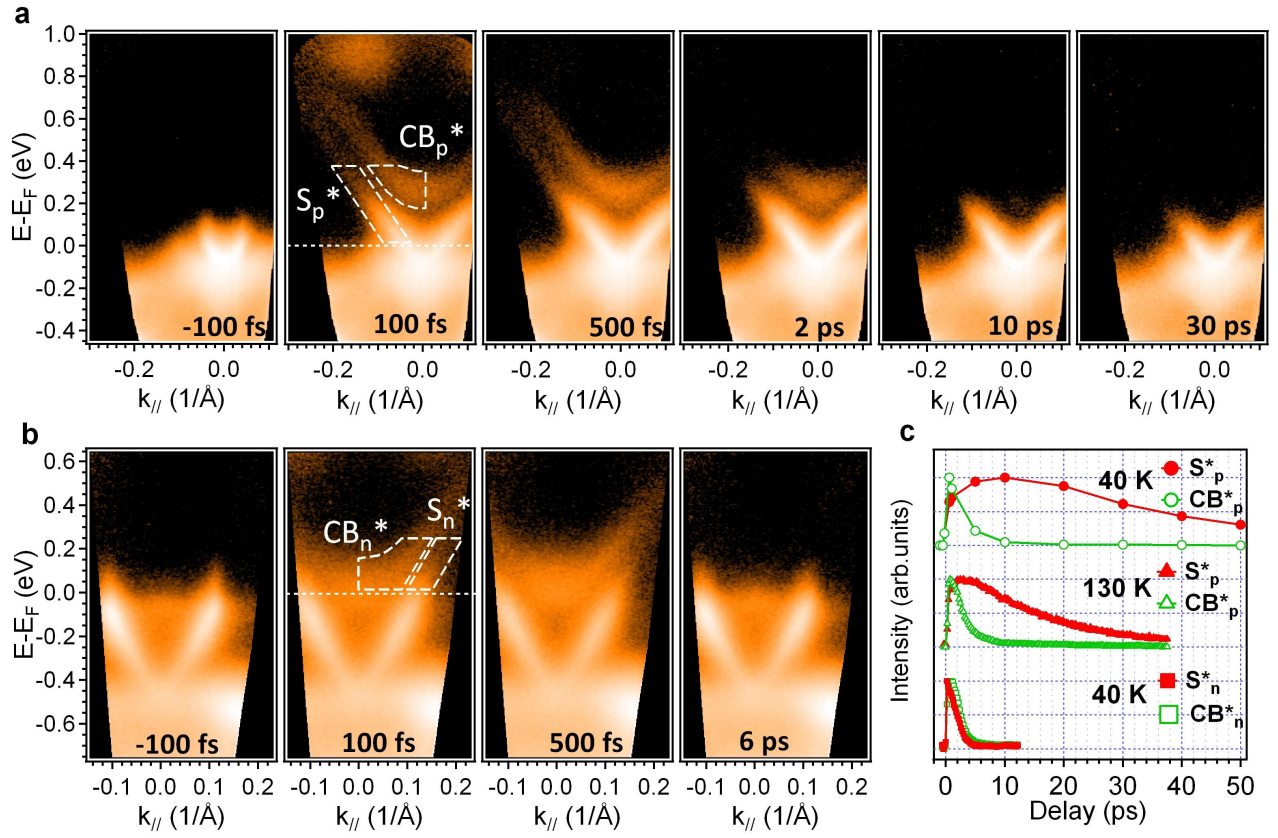
FIG. 1: Dirac cone ultrafast dynamics detected with time-resolved ARPES. Selected time delays are presented for (a) p-type \text{Bi}_{2.2}\text{Te}_3 and (b) n-type \text{Bi}_2\text{Te}_2\text{Se} . The signal intensity is presented in a logarithmic color scale. The integration regions called S_p^* , S_n^* , and CB_p^* , CB_n^* are indicated as dashed contour windows. (c) time evolution of S_p^* , S_n^* , CB_p^* , CB_n^* .
