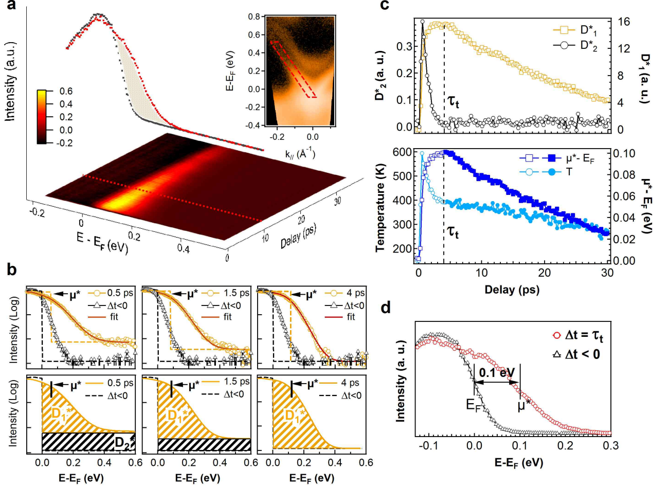
FIG. 6: Transient electronic temperature and chemical potential of non-equilibrium Dirac fermions. (a) Contour plot of the energy-time distribution of transient hot carriers in the surface Dirac cone of p-type \text{Bi}_{2.2}\text{Te}_3 at 130 K. The two spectra above the contour plot are two representative momentum-selected EDC's extracted from the integration area indicated in the inset, for \Delta t = 10 ps and \Delta t < 0 ps, respectively; the excess electron population is represented by the shaded area between them, and it corresponds to the color scale in the 2D plot. (b) Top panels: momentum-selected EDC's at \Delta t = 0.5 , 1.5 and 4 ps with relative fitting curves, and their difference with respect to the EDC taken at \Delta t < 0 ps; bottom panels: visualisation for the various time delays of D_1^* and D_2^* , parameters used to fit the transient electronic states with a Fermi-Dirac distribution as explained in the text. (c) Time evolution of the fitting parameters. (d) Comparison of the momentum-selected EDC's for the Dirac cone at equilibrium and for \Delta t = \tau_t
