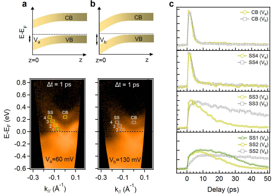
FIG. 4: Effect of band bending on the recombination rate for p-type \text{Bi}_{2.2}\text{Te}_3 Decay rates for photoexcited p- \text{Bi}_{2.2}\text{Te}_3 at T=40 K in the case of (a) a V_a=60 mV band bending and (b) of a V_b=130 mV band bending (b). The pump-probe ARPES images correspond to a time delay of 1 ps. In (c) the decay rates for equivalent energy windows are compared. The energy windows for the surface state SS have been chosen so that SS4 has from the same binding energy as the bottom of the conduction band CB. As it can be clearly seen, equivalent windows for the two surfaces show a much longer relaxation time for surface (b), where the band bending is more pronounced. In particular, SS2 for the case (b) has a lifetime \geq 100 ps (there is of course no equivalent in (b) of window SS1 because, due to the increased band bending, in (b) SS1 becomes part of the filled electronic states).
