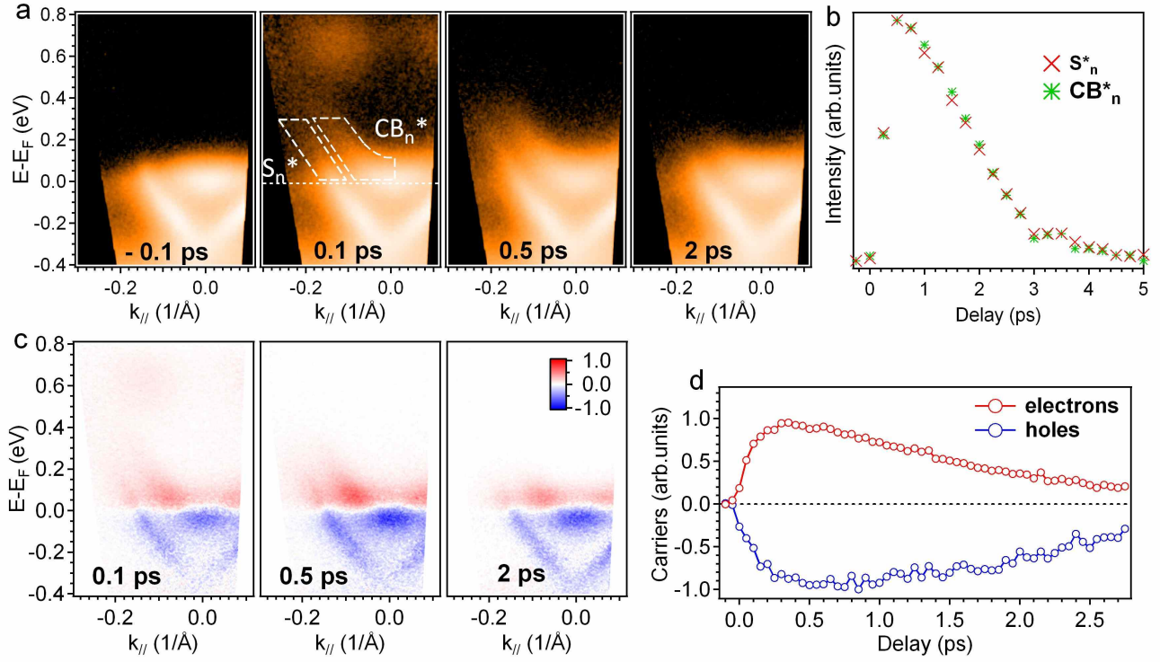
FIG. 2: Ultrafast dynamics of a flat-band, n-type \text{Bi}_2\text{Te}_3 sample. (a) Time-resolved ARPES images. (b) Time evolution of the electron populations in the Dirac cone and in the conduction band: as one can see, the relaxation time for excess electrons in the Dirac cone is much faster than for the p-type sample (see also Supplementary Figure S1), because in this case they are strongly coupled with the conduction band and they have access to the faster bulk carrier recombination channels. (c) k - E distribution of excess electrons and holes; (d) time evolution of the excess electron and hole populations. As expected for a flat band system, the electron and hole populations are very well balanced for all time delays: this becomes even more evident by comparing Fig. 2(c) and (d) with Fig. 3, where asymmetric populations are detected for excess holes and electrons, respectively.
