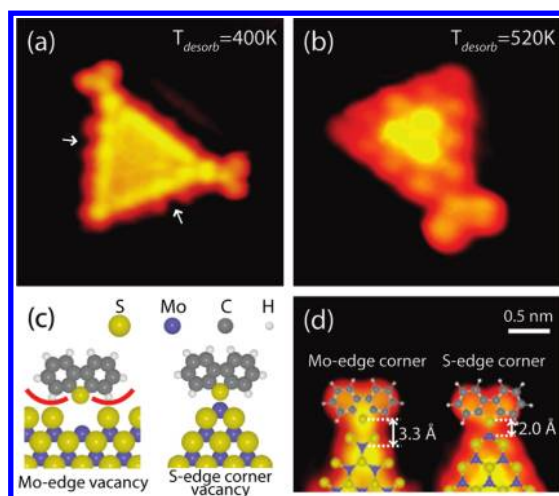
Figure 4. Adsorption of DBT on \text{MoS}_2 nanoclusters after exposure to atomic hydrogen. (a) Large ( n = 10 ) Mo-edge-terminated nanocluster after exposure to atomic hydrogen and DBT ( 56 \times 56 \text{ \AA}^2 ). (b) Small ( n = 4 ) S-edge-terminated nanocluster after exposure to atomic hydrogen and DBT ( 25 \times 25 \text{ \AA}^2 ). (c) DBT adsorption configurations on edge and corner vacancies on Mo edge and S edge clusters, respectively. (d) High-resolution STM images of DBT molecules on corner sites with the adsorption models superimposed on the STM images.
