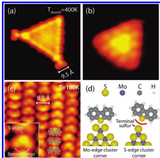
Figure 2. Adsorption of dibenzothiophene (DBT). (a) STM image ( 52 \times 52 \text{ Å}^2 ) of a Mo-edge-terminated cluster after dosing of DBT at 300 K. (b) S-edge-terminated cluster after dosing of DBT at 300 K. The image is 22 \times 22 \text{ Å}^2 . (c) DBT molecules on the virgin Au(111) surface at 180 K. The image is 50 \times 50 \text{ Å}^2 . The inset shows a close-up STM image ( 15 \times 15 \text{ Å}^2 ) of a DBT molecule. (d) Illustrations of the adsorption of DBT on the corner sites of Mo- and S-edge-terminated clusters.
