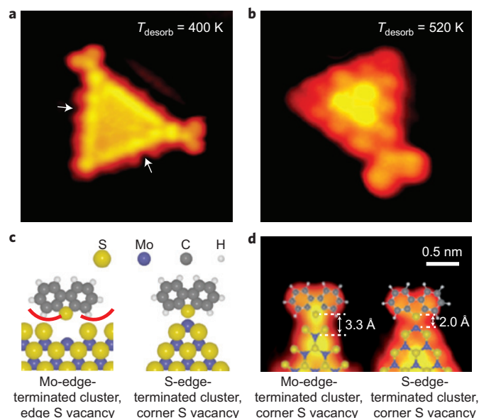
Figure 5 | Surface chemistry probed by adsorption of DBT. a , STM image (52 × 52 Å 2 ) of a Mo-edge-terminated cluster after dosing of DBT at 300 K. The white arrows indicate S vacancies. b , S-edge-terminated cluster after dosing of DBT at 300 K. The STM image is 22 × 22 Å 2 . c , Illustrations of the adsorption of DBT on sites of Mo-edge-terminated (edge, left) and S-edge-terminated (corner, right) clusters with S vacancies 70 . The red curves in the case of the Mo-edge cluster show steric hindrance. d , STM images (15 × 15 Å 2 ) of the corner sites of a Mo- and S-edge S vacancy sites interacting with a DBT molecule. The distances between the S atom of DBT and the corner Mo atom show that the shape of the MoS 2 material greatly influences its interaction with DBT, and the efficiency of its desulfurization. Figure reproduced with permission from ref. 70, © 2012 ACS.
