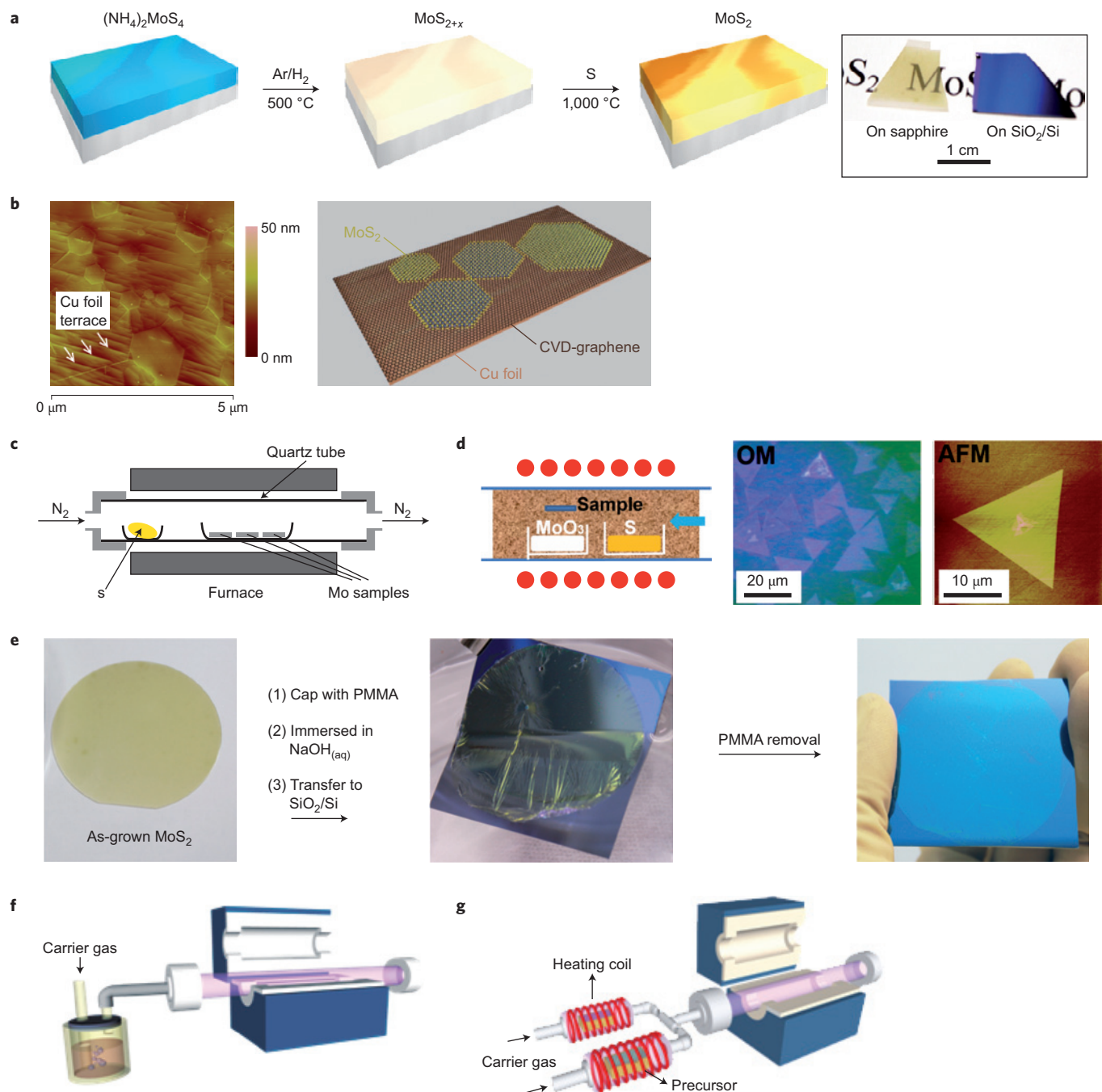
Figure 4 | Chemical vapour deposition of ultrathin TMDs. a , Schematic of \text{MoS}_2 layer deposited by two-step thermolysis, and the films obtained on a sapphire and silica substrate. 53 b , \text{MoS}_2 nanosheets on CVD graphene/Cu substrates through van der Waals epitaxy. 55 c , Schematic illustration of single- to few-layered \text{MoS}_2 by sulfurization of Mo thin film. 56 d , Alternative method for the growth of a \text{MoS}_2 monolayer, also on a substrate (sample) from \text{MoO}_3 and S powders through a gas-phase reaction. The substrate has been treated with aromatic molecules to assist the growth of larger flakes, as shown by the optical micrograph and atomic force microscopic images of the triangular nanosheets that are obtained. 57 The red circles represent the heating reaction chamber. e , Wafer-scale deposition of mono- to few-layered \text{MoS}_2 films obtained by direct sulfurization of \text{MoO}_3 thin films, and their transfer onto arbitrary substrates. 60 f, g , CVD of ultrathin TMDs by vaporization and decomposition of a single precursor in solution ( f ) and by vaporization and decomposition of metal and chalcogen precursors in solid forms ( g ). Figures reproduced with permission from: a , ref. 53, © 2012 ACS; b , ref. 55, © 2012 ACS; d , ref. 57, © 2012 Wiley; e , ref. 60, © 2012 RSC.
