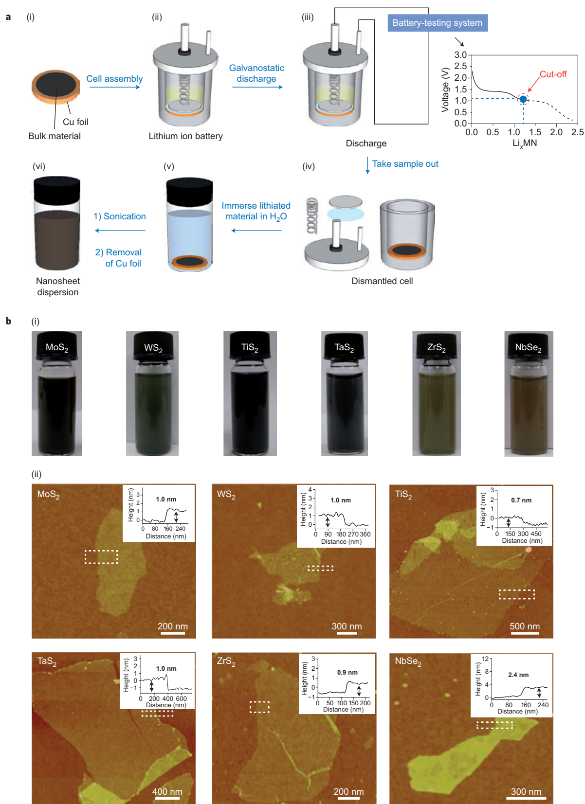
Figure 3 | Chemical exfoliation of monolayered TMDs. a , Schematic representation of the electrochemical lithiation process for synthesis of 2D nanosheets from layered bulk materials 47 . The cut-off voltage used to optimize the electrochemical lithiation conditions for preparation of few-layer BN, NbSe 2 , WSe 2 , Sb 2 Se 3 and Bi 2 Te 3 is also indicated. b , (i) Photographs of 2D nanosheet dispersions and (ii) the corresponding atomic force microscope images on SiO 2 substrates 42,47 . The insets of the AFM images represent height profiles from the substrate onto the nanosheets. The height of the step at the edge indicates the thickness of the nanosheets. Figures reproduced with permission from: a , b (i,ii) NbSe 2 , ref. 47, © 2012 Wiley; b (i) MoS 2 , WS 2 , TiS 2 , TaS 2 , b (ii) WS 2 , TiS 2 , TaS 2 , ZrS 2 , ref. 42, © 2011 Wiley.
