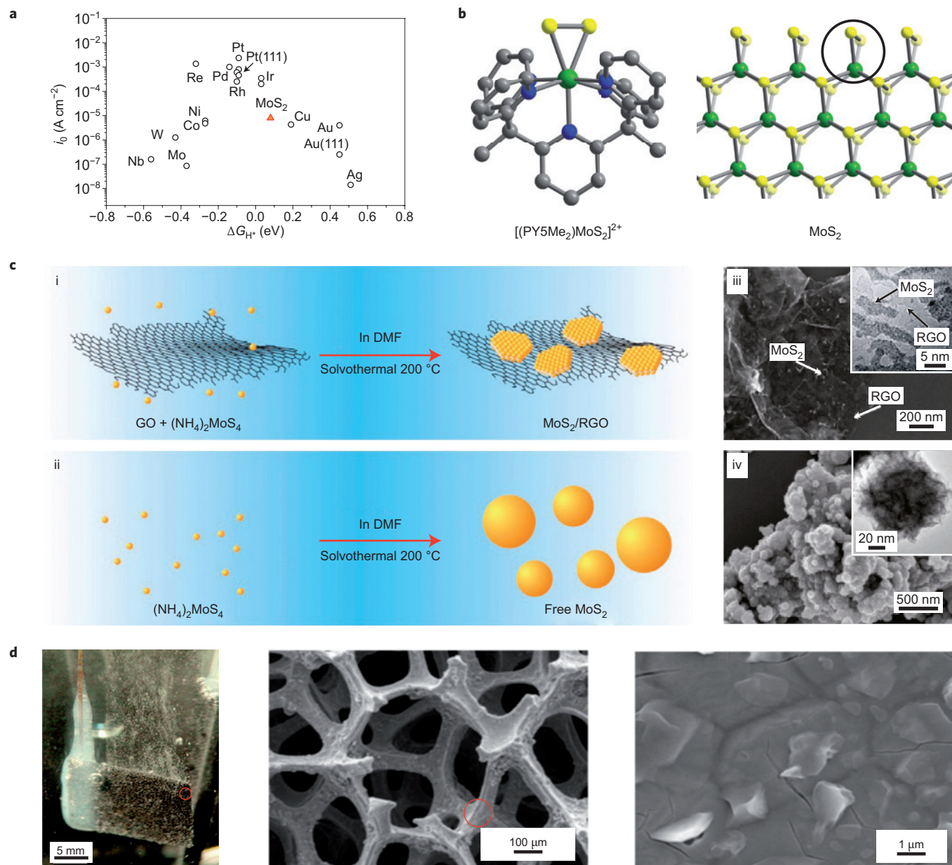
Figure 6 | Hydrogen evolution reaction catalysis with TMDs. a , Volcano plot of exchange current density ( i_0 ) as a function of DFT-calculated Gibbs free energy ( \Delta G_{\text{H}^+} ) of adsorbed atomic hydrogen for MoS 2 and pure metals 82 . b , [(\text{PY}_5\text{Me}_2)\text{MoS}_2]^{2+} compound designed to mimic the edges of MoS 2 . Colour code of the atoms: green, Mo; yellow, S; light blue, F; red, O; blue, N; and grey, C. H atoms are omitted for clarity 83 . c , (i, ii) Schematics of solvothermal synthesis (i) with graphene oxide sheets for MoS 2 /RGO hybrid synthesis and (ii) without graphene oxide sheets, resulting in large, free MoS 2 particles. (iii, iv) SEM and TEM (inset) images of the MoS 2 /RGO hybrid (iii) and of the free MoS 2 particles (iv) 75 . d , SEM images of graphene-protected Ni foam on which MoS 2 catalysts were grown 84 . Left, low magnification image of Ni foam coated with graphene and MoS 2 . Middle, the region indicated by the red circle in the left image has been magnified to show the skeleton structure of the foam. Right, magnified region from the red circle in the central image, showing the graphene/MoS 2 films on the polycrystalline Ni foam. Figures reproduced with permission from: a , ref. 82, © 2007 AAAS; b , ref. 83, © 2012 AAAS; c , ref. 75, 2011 ACS; d , ref. 84, © 2012 Wiley.
