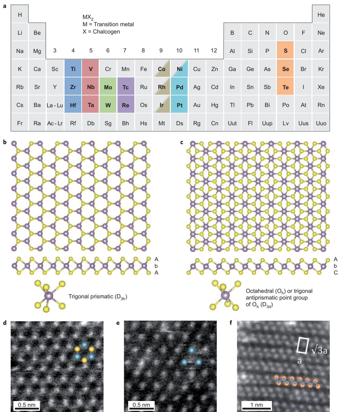
Figure 1 | Structure of monolayered TMDs. a , About 40 different layered TMD compounds exist. The transition metals and the three chalcogen elements that predominantly crystallize in those layered structure are highlighted in the periodic table. Partial highlights for Co, Rh, Ir and Ni indicate that only some of the dichalcogenides form layered structures. For example, NiS 2 is found to have apyrite structure but NiTe 2 is a layered compound. b,c , c-Axis and [11-20] section view of single-layer TMD with trigonal prismatic ( b ) and octahedral ( c ) coordinations. Atom colour code: purple, metal; yellow, chalcogen. The labels AbA and AbC represent the stacking sequence where the upper- and lower-case letters represent chalcogen and metal elements, respectively. d,e , Dark-field scanning transmission electron microscopy image of single-layer MoS 2 showing the contrast variation of 1H ( d ) and 1T ( e ) phases. Blue and yellow balls indicate Mo and S atoms, respectively. f , Zigzag chain clusterization of W atoms due to Jahn-Teller distortion in single layer WS 2 . The clustered W atoms are represented by orange balls. The \sqrt{3}a \times a unit cell of the superstructure is indicated with a white rectangle. Images in d and e reproduced with permission from ref. 12, © 2012 ACS. Image in f courtesy of T. Fujita.
