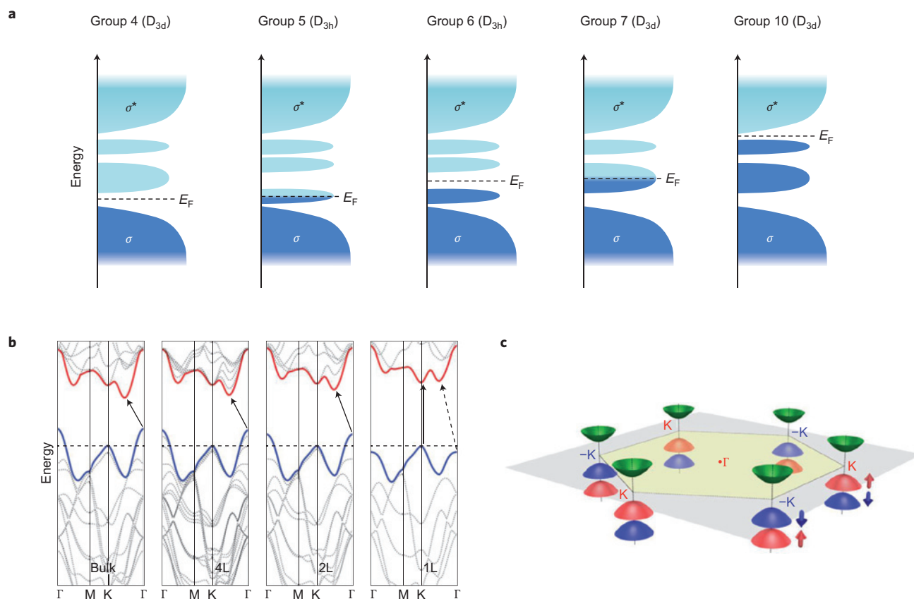
Figure 2 | d-Orbital filling and electronic character of various TMDs. a , Qualitative schematic illustration showing progressive filling of d orbitals that are located within the bandgap of bonding ( \sigma ) and anti-bonding states ( \sigma^* ) in group 4, 5, 6, 7 and 10 TMDs. D_{3h} and D_{3d} refer to the point group associated with the trigonal prismatic and the octahedral coordination of the transition metals (that is, the two monolayer polymorphs described in Fig. 1b). It should be noted that this simple model assumes ideal coordination; structural distortion often seen in many tellurides and group 7 TMDs lead to deviation in the electronic structure. The filled and unfilled states are shaded with dark and light blue, respectively. According to ligand field theory, D_{3d} compounds form two non-bonding d orbitals, d_{yz,xz,xy} (bottom) and d_{z^2,x^2-y^2} (top), while D_{3h} (or O_h ) compounds exhibit three d orbitals whose character is predominantly d_{z^2} , d_{x^2-y^2,xy} and d_{xz,yz} (from bottom to top). When an orbital is partially filled (such as in the case of group 5 and 7 TMDs), the Fermi level ( E_F ) is within the band and the compound exhibits a metallic character. When an orbital is fully filled (such as in group 6 TMDs), the Fermi level is in the energy gap and a semiconducting character is observed. b , Energy dispersion (energy versus wavevector k ) in bulk, quadrilayer (4L), bilayer (2L) and monolayer (1L) \text{MoS}_2 from left to right. The horizontal dashed line represents the energy of a band maximum at the K point. The red and blue lines represent the conduction and valence band edges, respectively. The lowest energy transition (indicated by the solid arrows) is direct (vertical) only in the case of a single layer. Indirect transition in monolayer (dashed arrow in 1L plot) is greater in energy than the direct band edge transition (solid arrow). c , Band structure of \text{MoS}_2 showing six valleys and opposite spin-orbit splitting of the valence band at the K and K' ( -K ) points. The red and blue surfaces represent spin-orbit-split valence band maxima, each of which is associated with a particular electron spin. The green surfaces represent the conduction band minima or the valleys. Figures reproduced with permission from: b , ref. 6, © 2010 ACS; c , ref. 36, © 2012 APS.
