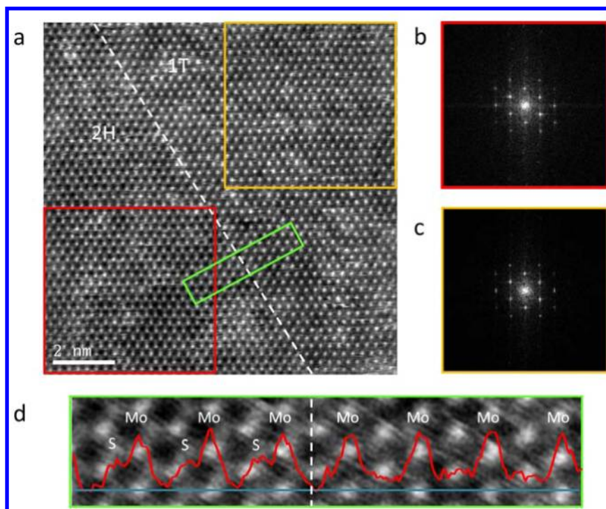
Figure 3. (a) STEM image of a region where a boundary between 2H (left) and 1T (right) phases is observed. The phase boundary is parallel to \{-1100\} planes and marked by a dashed line. (b, c) Fourier transform image of the (b) lower left and (c) upper right box of the STEM images. (d) Enlarged image of the region indicated by the green rectangle in image a. The intensity profile along the blue line is overlaid on the image. The width of the image corresponds to 3.9 nm.
