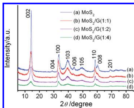
Figure 2. XRD patterns of (a) \text{MoS}_2 , (b) \text{MoS}_2/\text{G} (1:1), (c) \text{MoS}_2/\text{G} (1:2), and (d) \text{MoS}_2/\text{G} (1:4) prepared by hydrothermal route and annealing in \text{H}_2/\text{N}_2 at 800^\circ\text{C} for 2 h.
