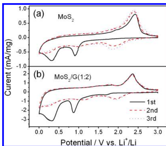
Figure 6. Cyclic voltammograms of (a) \text{MoS}_2 and (b) \text{MoS}_2/\text{G} (1:2) at a scanning rate of 0.5 mV/s during the first three cycles.
