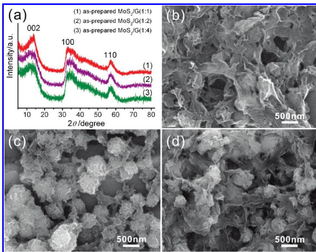
Figure 4. Characterizations of MoS 2 /G composites before annealing: (a) XRD patterns of (1) as-prepared MoS 2 /G (1:1), (2) as-prepared MoS 2 /G (1:2), (3) as-prepared MoS 2 /G (1:4), and the SEM images of (b) as-prepared MoS 2 /G (1:1), (c) as-prepared MoS 2 /G (1:2), and (d) as-prepared MoS 2 /G (1:4).
