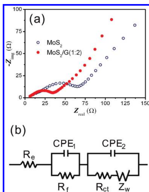
Figure 8. (a) Nyquist plots of \text{MoS}_2 and \text{MoS}_2/\text{G} (1:2) electrodes obtained by applying a sine wave with amplitude of 5.0\text{ mV} over the frequency range from 100\text{ kHz} to 0.01\text{ Hz} ; (b) equivalent circuit model of the studied system. CPE represents the constant phase element, Z_{\text{CPE}} = \{Q(j\omega)^n\}^{-1} , 0 \leq n \leq 1 .
