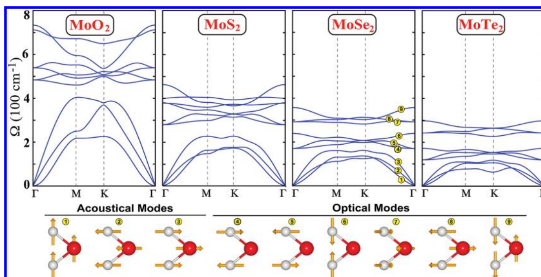
Figure 6. Calculated phonon branches of stable H structures of \text{MoX}_2 ( X = \text{O}, \text{S}, \text{Se}, \text{and Te} ) compounds along the \Gamma\text{--M--K--}\Gamma directions of the BZ. Phonon branches are labeled by numerals. The acoustical and optical phonon modes at the \Gamma point are depicted in the bottom panel. All branches are presented using the same scale of frequency.
