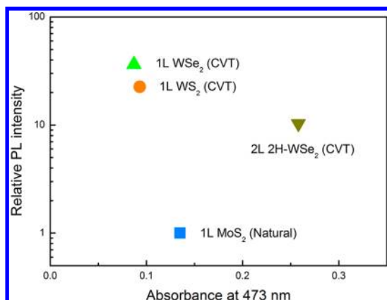
Figure 5. Relative integrated PL intensity of \text{WS}_2 and \text{WSe}_2 monolayers and \text{WSe}_2 bilayer with respect to that of a \text{MoS}_2 monolayer plotted against absorbance at the excitation wavelength of 473 nm. The PL emission spectra were integrated over 520–950 nm. Absorbance is obtained from differential reflectance of samples on quartz based on eq 1. The absorbance of \text{MoS}_2 is obtained from ref 5. Note that the comparison is made between exfoliated samples from synthetic ( i.e. , CVT-grown) \text{WS}_2/\text{WSe}_2 and natural \text{MoS}_2 (SPI supplies) crystals.
