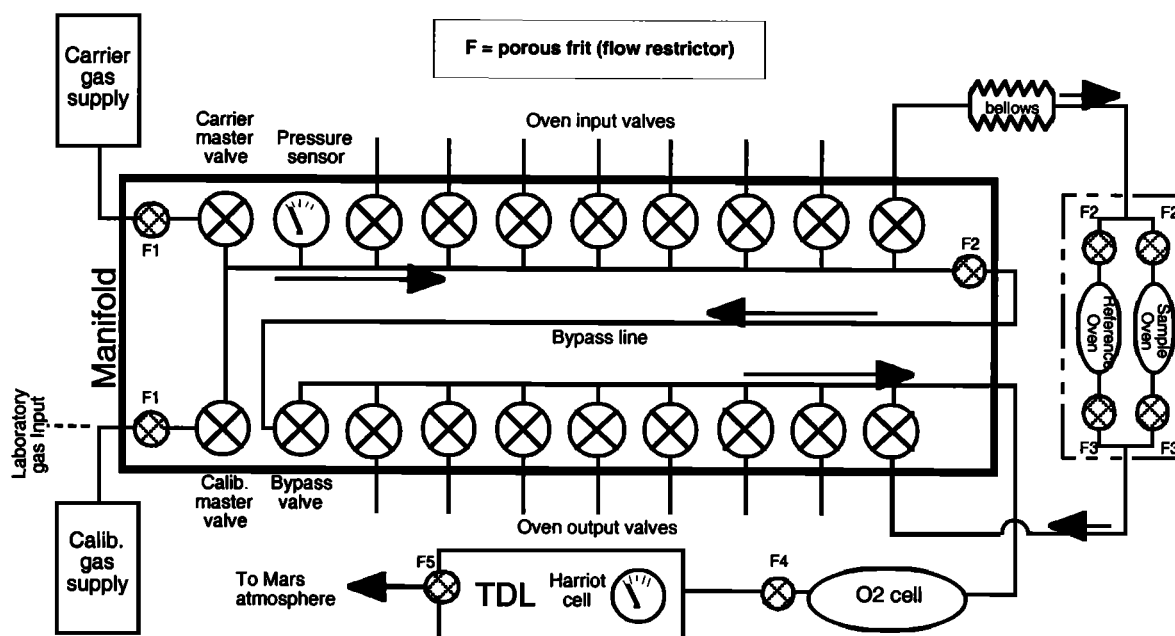
Figure 4. TEGA gas-handling system. Actuation of one of the master valves determines whether carrier or calibration gas is introduced into the system. Controlled, cyclic actuation of the master valve serves as a simple regulator of the pressure, which is monitored by the sensor on the manifold. Each oven pair has an inlet and outlet valve to control the flow of gas and a frit at each end to contain the sample. Additional frits are provided as shown to produce different pressures in the EGA cells. The bypass line is used to supply calibration gas to the EGA cells and to purge them following calibration.
