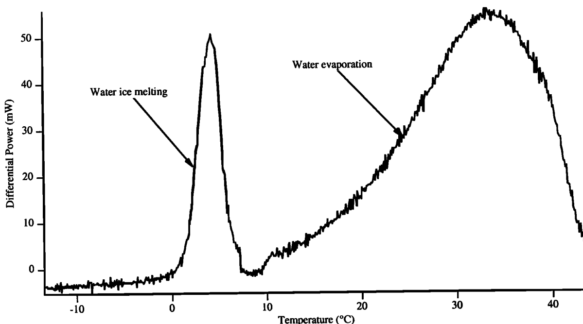
Figure 8. The melting and evaporation of 10 mg of water was observed in an end-to-end system test. Clear separation between the two processes is observed.
