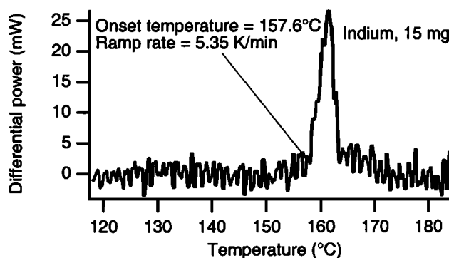
Figure 6. Determination of the onset temperature and the enthalpy for a pure sample as illustrated by a TEGA EQM run with a 15 mg sample of indium. The onset temperature is defined as the intersection of the baseline and a straightline fit to the leading edge of the peak. The enthalpy change of the sample corresponds to the area of the peak when power is plotted against time. The noisy data are due to a nonoptimized control law (see text).
