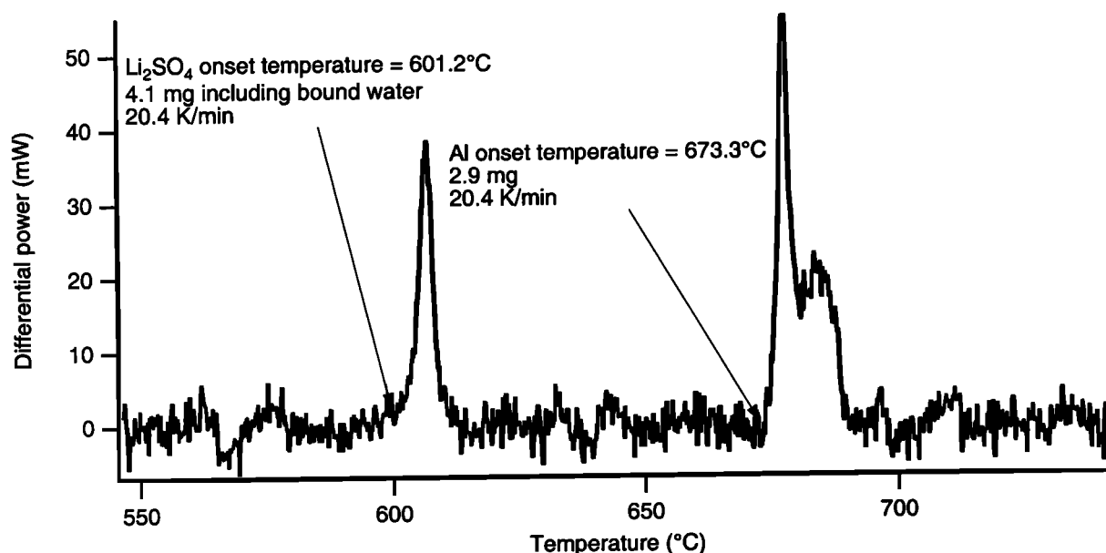
Figure 7. Calibration run with lithium sulfate and aluminum in the TEGA EQM. This run and the indium run were used to establish the temperature and caloric calibration of the TEGA DSC. The noisy data are due to a nonoptimized control law (see text).
