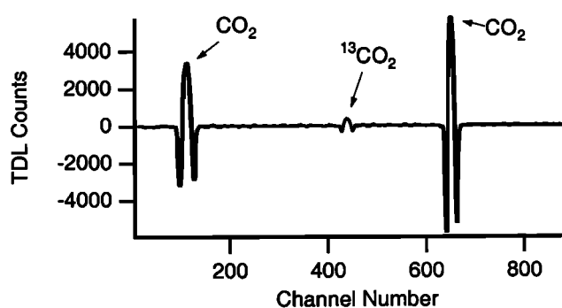
Figure 5. The 2f spectrum of the FM CO 2 TDL illustrating the relative signal strengths of the 12 CO 2 and 13 CO 2 lines. For this spectrum, pure CO 2 was flowing in the TDL cell with the terrestrial ratio of 13 CO 2 to 12 CO 2 .
