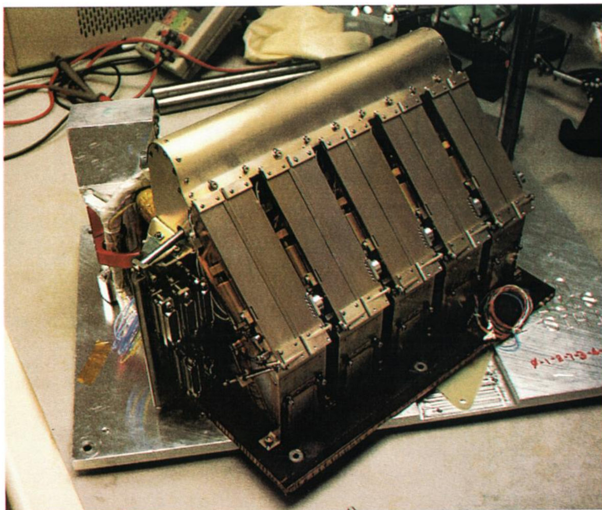
Plate 1. Flight model of the Thermal and Evolved Gas Analyzer. Five of the eight one-use thermal analyzer modules are visible. The carrier and calibration gas tanks, gas handling system, oxygen sensor, diode-matrix switching board, and wiring management system are housed between the bank of five thermal analyzers shown and the bank of three analyzers not in view on the opposite side of the instrument. The tunable diode laser spectrometer is on the left in a separate housing with its cover removed. For scale, each thermal analyzer module is 38 mm wide.
