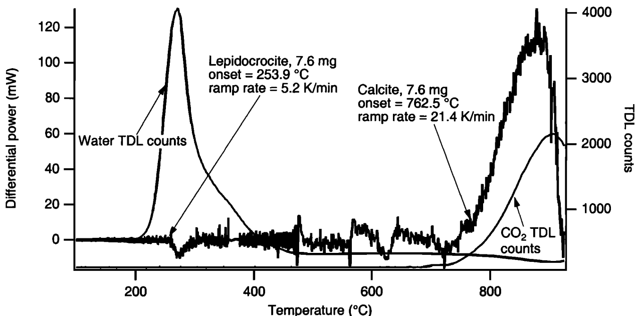
Figure 9. Sample run in the TEGA EQM. Lepidocrocite, pyrolusite, and calcite demonstrate the detection of multiple thermal transitions and their associated gas releases. Lepidocrocite releases water as it transforms into maghemite, and calcite releases CO 2 during its decomposition. The DSC data were taken before we optimized the control law to reduce noise.
