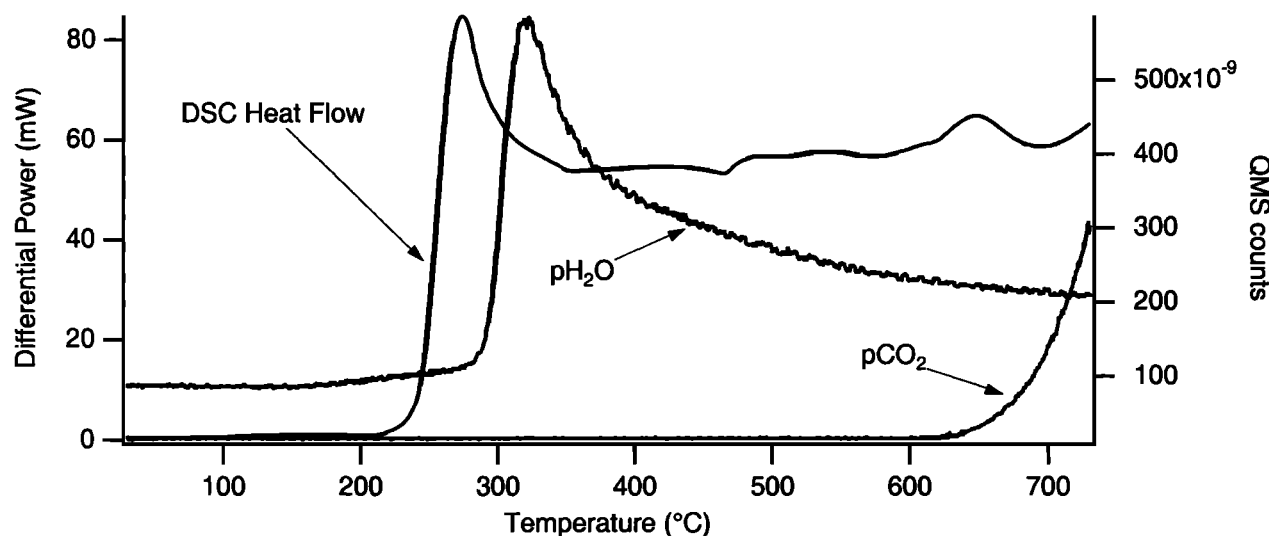
Figure 10. Lepidocrocite, pyrolucite, and calcite sample run in Perkin-Elmer laboratory DSC. Evolved gas detection was performed with a quadrupole mass spectrometer. The full calcite transition occurs at temperatures higher than the maximum instrument temperature.
