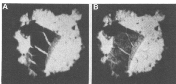
Fig. 3. Effect of heating on the high-pressure, room-temperature phase. (A) Before the heating (20 GPa). Although the whole sample has already transformed to the high-pressure phase, the sample is too thick to allow us to observe the transmissivity of light except the thin edges. (B) After heating by a YAG laser. The transmissivity of light increased drastically.
