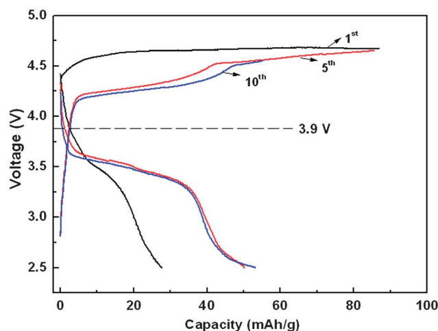
Fig. 10 The 1st, 5th and 10th charge–discharge profiles of the \text{Na}_3\text{NiZr}(\text{PO}_4)_3/\text{Na} batteries.
