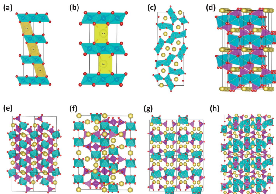
Fig. 21 The crystalline structure of several available cathode materials for Na-ion batteries. (a) O3-NaMO 2 , (b) P2-NaMO 2 , (c) Na 0.44 MnO 2 , (d) olivine NaFePO 4 , (e) Na 2 FeP 2 O 7 , (f) NASICON-Na 3 V 2 (PO 4 ) 3 , (g) Na 2 FePO 4 F, (h) Na 4 Fe 3 (PO 4 ) 2 P 2 O 7 .
