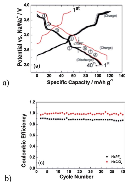
Fig. 6 (a) Galvanostatic curves of P2-Na 0.74 CoO 2 /NaPF 6 /Na cells at a current rate of C/10 and (b) coulombic efficiency of the cells as a function of the cycle number. Reprinted from J. J. Ding, Y. N. Zhou, Q. Sun, X. Q. Yu, X. Q. Yang and Z. W. Fu, Electrochemical properties of P2-phase Na 0.74 CoO 2 compounds as cathode material for rechargeable sodium-ion batteries, Electrochim. Acta , 2013, 87 , 388–393, Copyright 2013, with permission from Elsevier.
