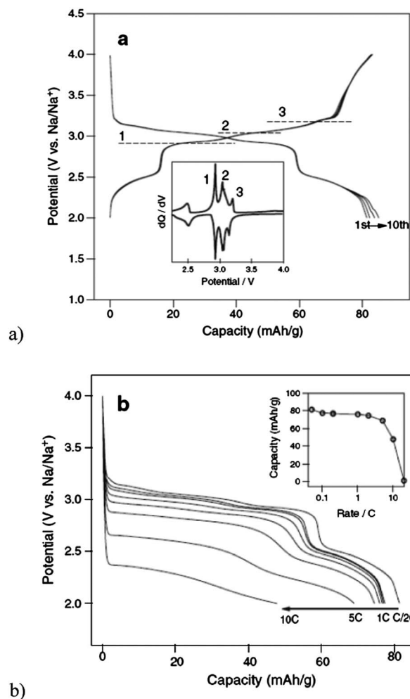
Fig. 20 (a) Galvanostatic voltage-composition curve at C/20 and (b) discharge capacity of \text{Na}_2\text{FeP}_2\text{O}_7 at different rates. Reprinted from P. Barpanda, T. Ye, S.-I. Nishimura, S.-C. Chung, Y. Yamada, M. Okubo, H. Zhou and A. Yamada, Sodium iron pyrophosphate: A novel 3.0 V iron-based cathode for sodium-ion batteries, Electrochem. Commun. , 2012, 24 , 116–119. Copyright 2012, with permission from Elsevier.
