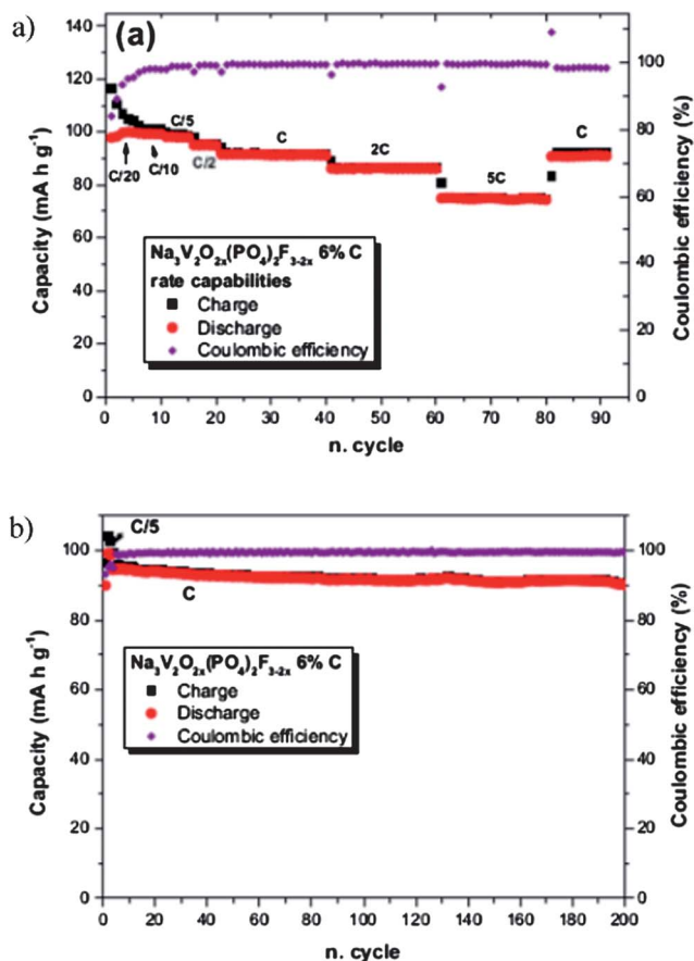
Fig. 15 (a) Specific charge/discharge capacity of Na 3 V 2 O 2x (PO 4 ) 2 F 3-2x at different C rates; and (b) cycling stability of Na 3 V 2 O 2x (PO 4 ) 2 F 3-2x over 200 cycles with a charge/discharge rate of C. The first 3 cycles were recorded with C/5. Reprinted from P. Serras, V. Palomares, A. Goñi, P. Kubiak and T. Rojo, Electrochemical performance of mixed valence Na 3 V 2 O 2x (PO 4 ) 2 F 3-2x /C as cathode for sodium-ion batteries, J. Power Sources , 2013, 241 , 56–60. Copyright 2013, with permission from Elsevier.
