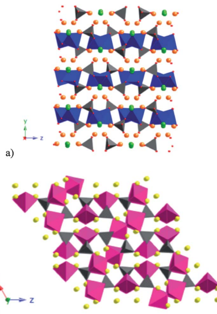
Fig. 16 Structures of (a) Na 2 FePO 4 F and (b) Na 2 MnPO 4 F.
