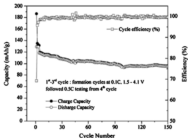
Fig. 8 Long term cycling and coulombic efficiency of Na-ion \text{Na}_{0.33}\text{C}/\text{Na}_{1-y}(\text{Ni}_{1/3}\text{-Fe}_{1/3}\text{Mn}_{1/3})\text{O}_2 cell. Following the 4 th cycle, the full cell was continuously cycled at a charge-discharge 0.5 C rate ( 75 \text{ mA g}^{-1} ) between 1.5 and 4.1 V. Reprinted from D. Kim, E. Lee, M. Slater, W. Lu, S. Rood and C. S. Johnson, Layered \text{Na}[\text{Ni}_{1/3}\text{Fe}_{1/3}\text{Mn}_{1/3}]\text{O}_2 cathodes for Na-ion battery application, Electrochem Commun. , 2012, 18 , 66–69, Copyright 2012, with permission from Elsevier.
