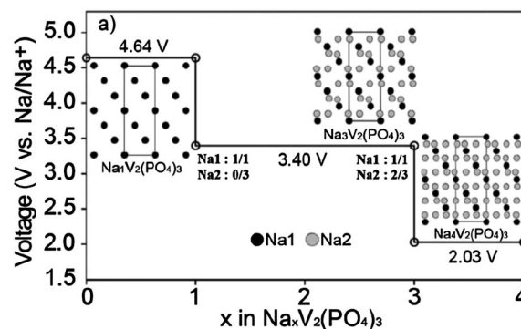
Fig. 11 Voltage profiles estimated from first principle calculations. Reproduced by permission of The Electrochemical Society from S. Y. Lim, H. Kim, R. A. Shakoar, Y. Jung and J. W. Choi, J. Electrochem. Soc. , 2012, 159 , A1393–A1397.
