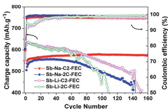
Fig. 33 Cycling performance of Sb electrode vs. \text{Na}^+ and \text{Li}^+ at C/2 and 2C with 5% FEC additive. Reprinted with permission from A. Darwiche, C. Marino, M. T. Sougrati, B. Fraisse, L. Stievano and L. Monconduit, J. Am. Chem. Soc. , 2012, 134 , 20805–20811. Copyright 2012 American Chemical Society.
