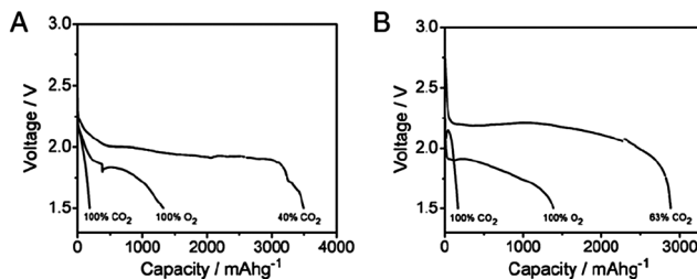
Fig. 37 Galvanostatic discharge profiles for Na-CO 2 /O 2 cells operated with different O 2 /CO 2 feeds by using (a) 0.75 M NaTFSI in ENIM Otf ionic liquid electrolyte, and (b) 1 M NaClO 4 in TEGDME tetraglyme electrolyte. Reprinted from S. K. Das, S. Xu and L. A. Archer, Carbon dioxide assist for non-aqueous sodium-oxygen batteries, Electrochem. Commun. , 2013, 27 , 59–62. Copyright 2013, with permission from Elsevier.
