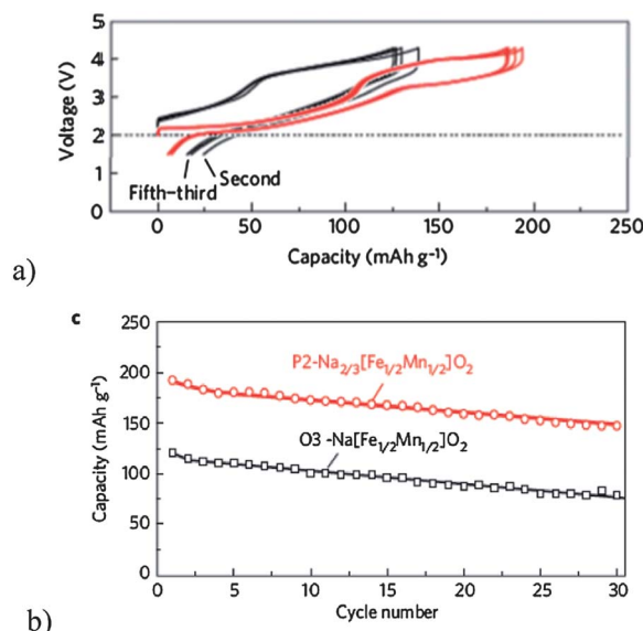
Fig. 7 (a) Galvanostatic charge/discharge (oxidation/reduction) curves for Na/Na[Fe 1/2 Mn 1/2 ]O 2 and Na/Na 2/3 [Fe 1/2 Mn 1/2 ]O 2 cells at a rate of 12 mA g -1 in the voltage range of 1.5 and 4.3 V; and (b) comparison of the discharge capacity retention of the sodium cells. Reprinted by permission from Macmillan Publishers Ltd: N. Yabuuchi, M. Kajiyama, J. Iwatate, H. Nishikawa, S. Hitomi, R. Okuyama, R. Usui, Y. Yamada and S. Komaba, Nat. Mater. , 2012, 11 , 512–517. Copyright 2012.
