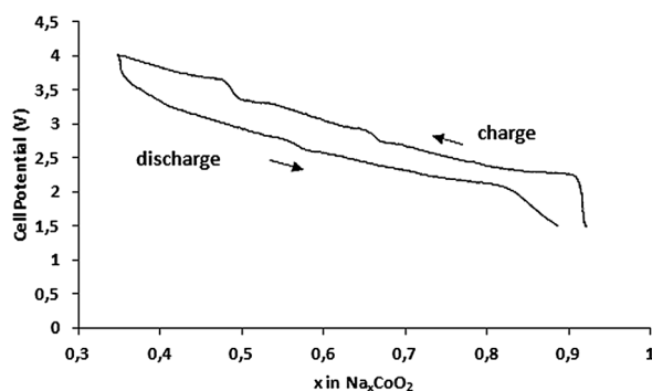
Fig. 2 Cell potentials vs. x for \text{Na}_x\text{CoO}_2 in a cell with a sodium anode and a \text{P}(\text{EO})_8\text{NaCF}_3\text{SO}_3 electrolyte at 90 °C. The current density was 0.5 \text{mA cm}^{-2} . Reproduced by permission of The Electrochemical Society from ref. 11.
