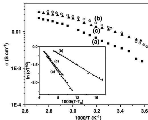
Fig. 25 Ionic conductivity as a function of temperature for the blends of ionic liquid/PVdF-HFP (a) 3 : 1 w/w; (b) 4 : 1 w/w; and (c) ionic liquid/PVdF-HFP (1 : 1 w/w) + \text{NaTf} gel polymer electrolyte. Reprinted from: D. Kumar and S. A. Hashmi, Ionic liquid based sodium ion conducting gel polymer electrolytes, Solid State Ionics , 181 , 416–423, Copyright 2010, with permission from Elsevier.
