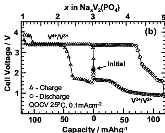
Fig. 21 Electrochemical charge-discharge curves for the \text{Na}_3\text{V}_2(\text{PO}_4)_3//1 \text{ M NaClO}_4/\text{PC}/\text{Na} cells at room temperature. Reproduced by permission of The Electrochemical Society from ref. 58.
