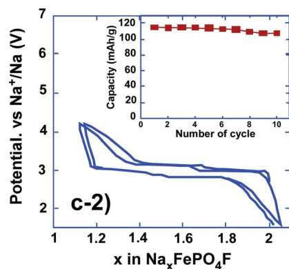
Fig. 17 Galvanostatic cycling vs. \text{Na}/\text{Na}^+ of the \text{Na}_2\text{FePO}_4\text{F} material synthesized by the ionothermal process at C/15 rate. Inset: Cyclability of \text{Na}_2\text{FePO}_4\text{F} . Reproduced by permission of The Electrochemical Society from ref. 47.
