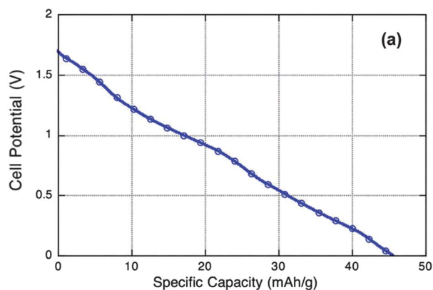
Fig. 5 Discharge profile of a \text{Na}_{0.44}\text{MnO}_2/\text{activated carbon} cell at C/8 . Reprinted from: J. F. Whitacre, A. Tevar and S. Sharma, \text{Na}_4\text{Mn}_9\text{O}_{18} as a positive electrode material for an aqueous electrolyte sodium-ion energy storage device, Electrochemistry Communications , 12 , 463–466, Copyright 2010, with permission from Elsevier.
