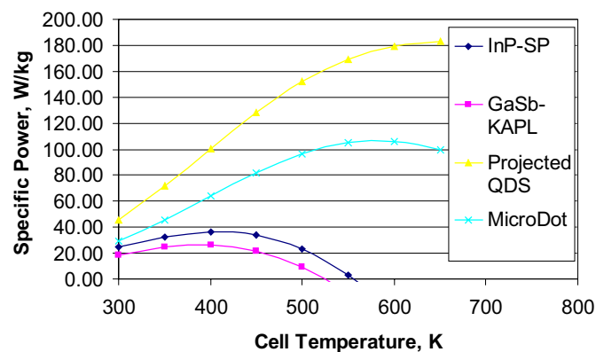
FIGURE 5. TPV Converter Module Specific Power with Radiator.
