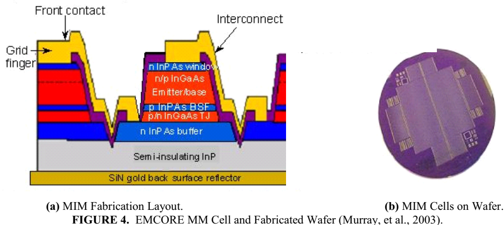
FIGURE 4. EMCORE MM Cell and Fabricated Wafer (Murray, et al., 2003).
