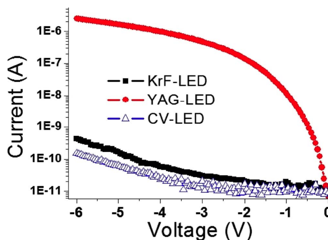
Figure 3. (Color online) Leakage currents of LEDs under a reverse bias of -5 \text{ V} .
