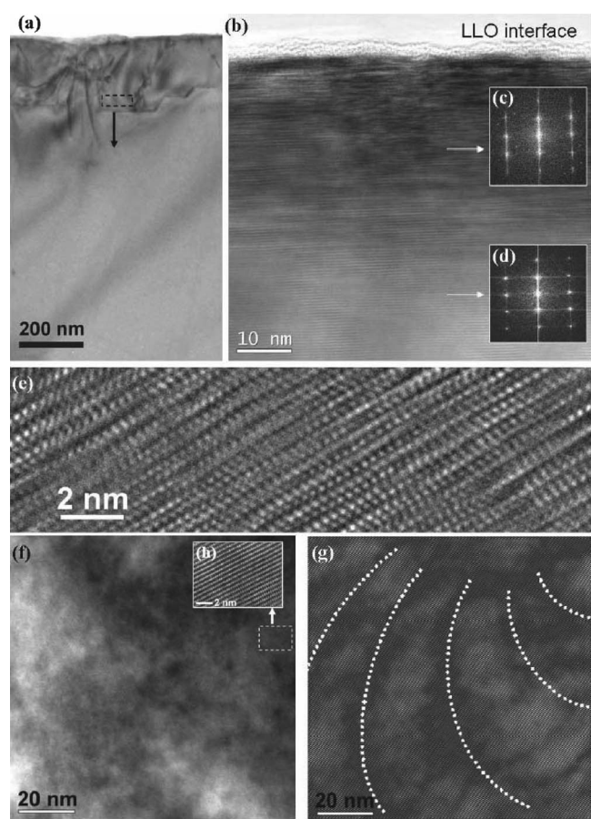
Figure 6. TEM images of the KrF-LED: (a) bright-field cross-sectional image of the KrF-LED LLO interface, (b) magnified part of the superficial region from (a), [(c) and (d)] fast Fourier transforms of different regions indicated by arrows, (e) HRTEM lattice image of the region 200 nm below the LLO interface, (f) TEM image of the region 200 nm from (a), (g) inversed fast Fourier transform image of (f) using diffraction spots along the [0002] direction, and (h) HRTEM lattice image of the region indicated by arrow.
