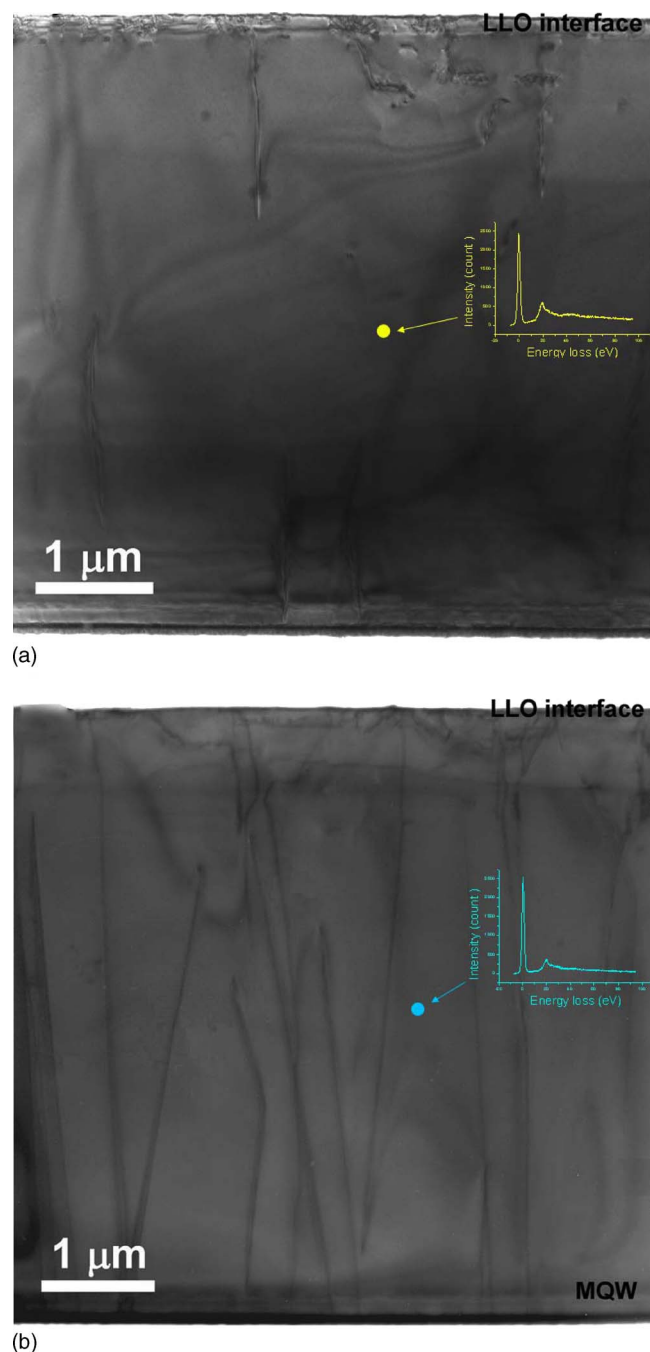
Figure 4. (Color online) TEM images of the whole LED structure: (a) KrF-LED and (b) YAG-LED.
