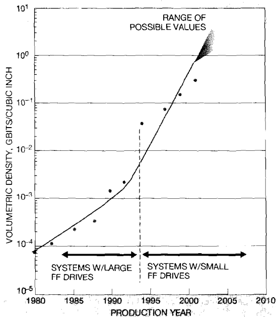
Figure 5 Storage system volumetric density trend
