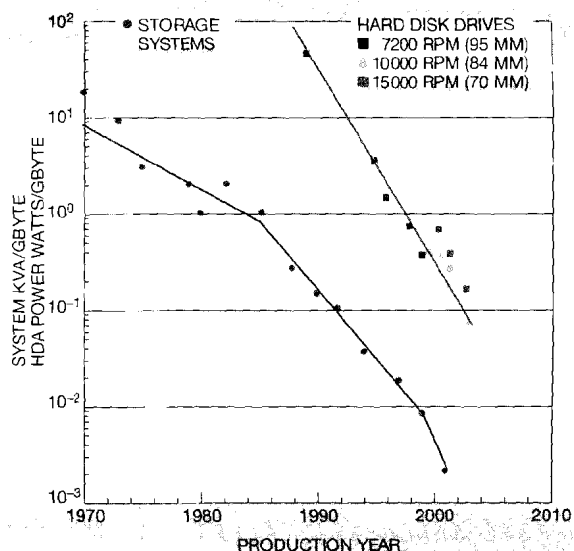
Figure 9 Hard disk drive and storage system power trend per Gbytes stored
