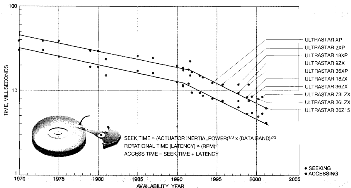
Figure 11 Disk drive access/seek times
