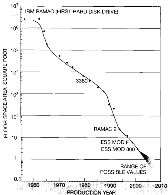
Figure 3 Floor space required to store 1 terabyte
