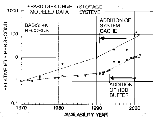
Figure 12 Performance trend for hard disk drives and storage systems
