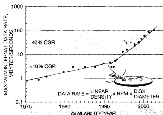
Figure 10 Hard disk drive maximum internal data rate for enterprise/server drives
