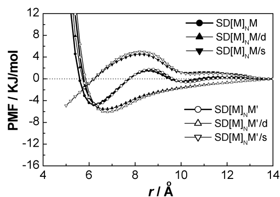
Fig. 8 The same as for Fig. 6 but for the cases \text{SD}[\text{M}]_{\text{N}}\text{M} and \text{SD}[\text{M}]_{\text{N}}\text{M}' .
