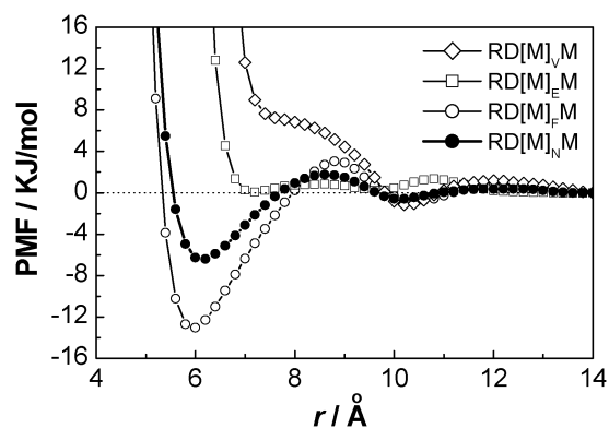
Fig. 5 As for Fig. 4 but for the rigid DWC with different orientations. The data points for RD[M] V M with r_c \leq 5.8 \text{ Å} and for RD[M] E M with r_c \leq 5.2 \text{ Å} are unavailable because the too-near constraint distances lead simulations to collapse.
