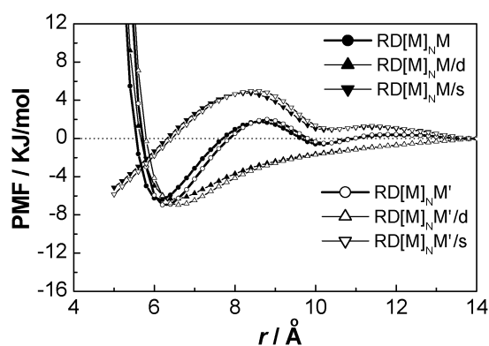
Fig. 6 Comparison of PMFs for the cases \text{RD}[\text{M}]_{\text{N}}\text{M} and \text{RD}[\text{M}]_{\text{N}}\text{M}' . These are decomposed into the direct cage-methane contribution (/d) and the solvent-induced contribution (/s). Error bars, not shown here for clarity, are similar to those in Fig. 3, except that the error bars for the direct cage-methane contribution are obscured by the symbols.
