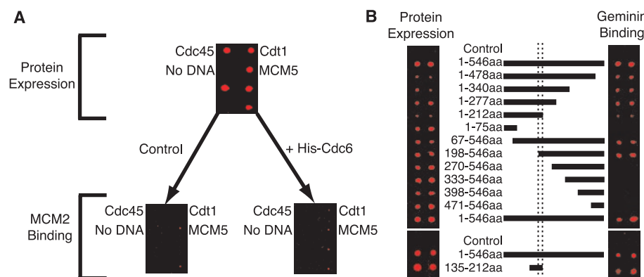
Fig. 4. Characterization of Cdt1. (A) Cdt1 regulation. NAPPAs was used to test whether Cdc6 could act as a bridging protein between Cdt1 and MCM2. Target proteins Cdt1, Cdc45 (negative control), and MCM5 (positive control) were expressed in duplicate (top panel) and confirmed by an antibody to GST. The target proteins were probed with either HA-MCM2 alone (left panel) or in the presence of coexpressed His-Cdc6 (right panel). The binding of MCM2 was detected with an antibody to HA. (B) Cdt1 deletion mapping. NAPPAs was used to map the binding domain of geminin on Cdt1. Fragments from various regions of Cdt1 (as indicated) were generated by PCR and cloned into target expression vectors. The partial or full-length polypeptides were expressed and detected on the array with an antibody to GST (left panel). To identify the binding region of geminin, the array was queried with HA-geminin (right panel) and developed with an antibody to HA. Vertical lines (dashed) delimit the small (15-aa) region common to all the fragments that bound geminin. A small 78-aa domain (135 to 212 aa) containing the noted 15 aa (198 to 212 aa) was expressed along with full-length Cdt1 (bottom left), which was again queried with geminin (bottom right).
