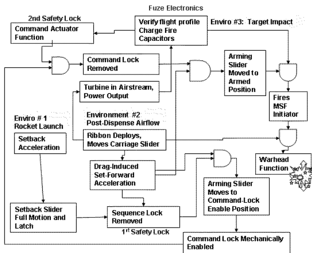
Fig. 2 Safety Logic Flow-chart
