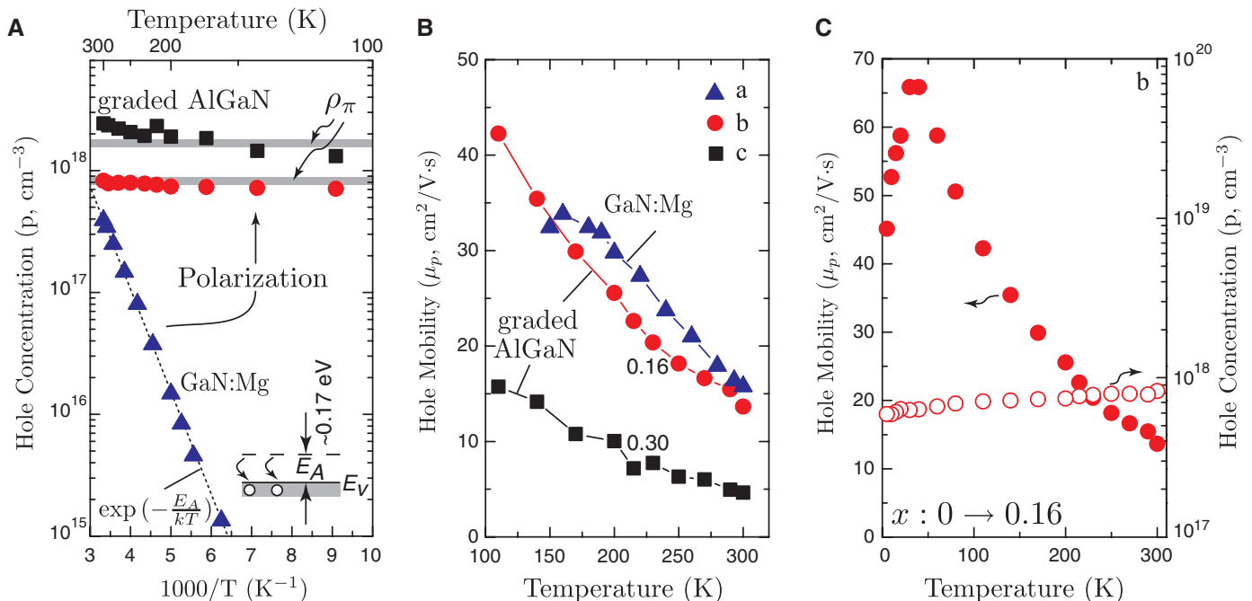
Fig. 3. Hall-effect temperature-dependent (A) hole concentration, (B) hole mobilities, and (C) hole concentration and mobility measured down to T = 4 K. The polarization-doped graded AlGa N p-type layers show higher hole
