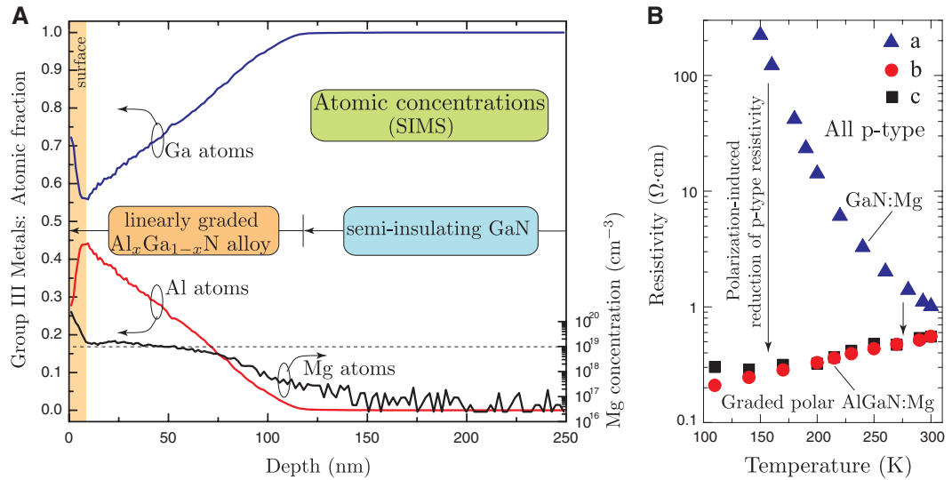
Fig. 2. Structural and transport properties of p-type samples (A) Concentration of Al and Ga atoms in a compositionally graded AlGa N sample (sample d), with the measured concentration of Mg dopant atoms. The thickness of the graded layer is d \sim 85 nm, capped with a thin, heavily doped p++ layer for ohmic contacts. SIMS, secondary ion mass spectrometry. (B) Measured temperature-dependent resistivity for samples a to c, highlighting the polarization boost in p-type conductivity.
