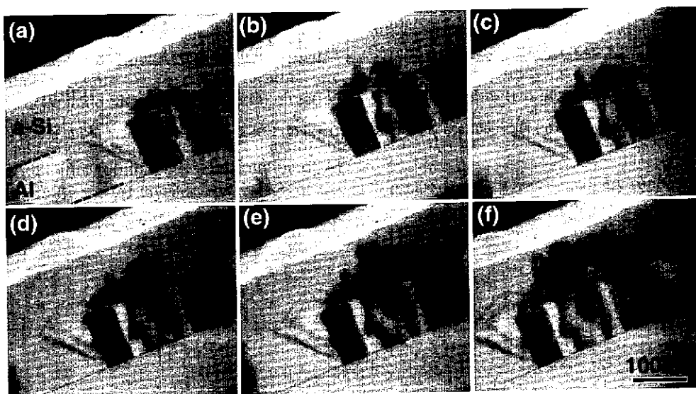
Fig. 3 A series of BF-TEM images of a-Si/Al film taken during in-situ heating at 553 K (average time interval 15 s).
