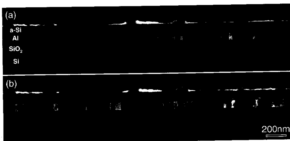
Fig. 4 BF-TEM images of a-Si/Al film. (a) as-deposited and (b) in-situ heated at 473 K for 0.3 ks.
