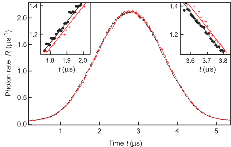
Fig. 3. Vacuum-induced group delay of a probe pulse. The black circles show the probe pulse in the absence of atoms; the red crosses indicate the probe pulse traveling through the atomic medium on VIT resonance \Delta = \delta = 0 . The observed delay induced by the cavity vacuum field is \tau = 25 \pm 2 \text{ ns} . The delayed pulse experiences absorption and has been rescaled by a factor of 1.6 for easier visualization of the group delay.
