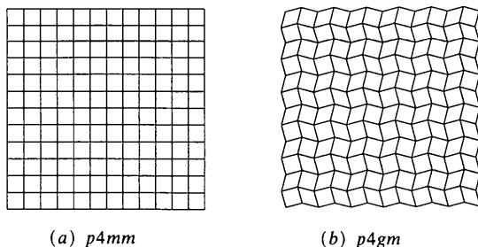
Fig. 2. The analogous crystallographic tilings with (a) symmorphic and (b) non-symmorphic space groups for the point group 4mm .
