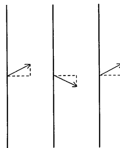
Fig. 6. The tiling vectors \mathbf{a} \pm \mathbf{c} for the non-symmorphic construction described in §II.B.
