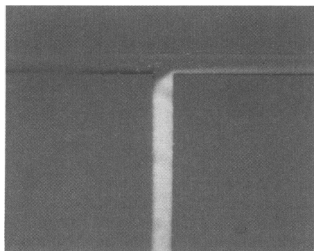
Fig. 4. Photomicrograph of a device with 10 kV (1 kV/cm) applied along the horizontal channel, while the side channel (vertical in the photo) was left floating. The potential drove buffer solution (pH 9.1) from left to right and caused a 100 \mu M fluorescein dye solution in the side channel (vertical in the figure) to be pulled in the direction of flow. The channels are 30 \mu m wide.
