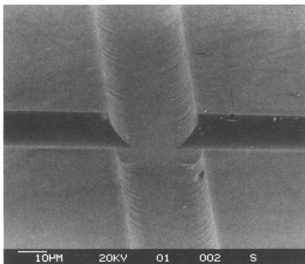
Fig. 1. Electron micrograph of capillary channels etched into Corning 7740 glass to a depth of 10 \mu m.
