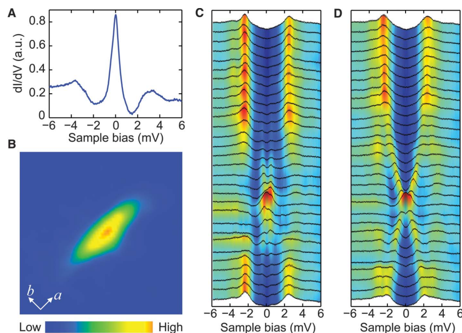
Fig. 2. The vortex core states. (A) STS (setpoint, 10 mV, 0.1 nA) on the center of a vortex core. (B) Zero-bias conductance map ( 40 \times 40 \text{ nm}^2 ; setpoint, 10 mV, 0.1 nA) for a single vortex at 0.4 K and 1 T magnetic field. (C and D) Tunneling conductance curves measured at equally spaced (2 nm) distances along a and b axes.
