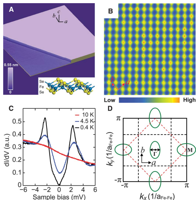
Fig. 1. STM characterization of the as-grown FeSe films. (A) Topographic image (2.5 V, 0.1 nA, 200 by 200 nm 2 ) of a FeSe film ( \sim 30 unit cells thick). The step height is 5.5 Å. (Inset) The crystal structure. (B) Atomic-resolution STM topography (10 mV, 0.1 nA, 5 by 5 nm 2 ) of FeSe film. The bright spots correspond to the Se atoms in the top layer. a and b correspond to either of Fe-Fe bond directions. The same convention is used for a and b axes throughout. (C) Temperature dependence of differential conductance spectra (setpoint, 10 mV, 0.1 nA). (D) Schematic of the unfolded Brillouin zone and the Fermi surface (green ellipses). The nodal lines for \cos k_x \cos k_y and (\cos k_x + \cos k_y) gap functions are indicated by black and red dashed lines, respectively. The sizes of all pockets are exaggerated for clarity. The black arrow indicates the direction of nesting.
