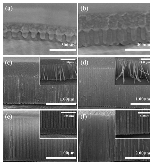
Fig. 2 SEM images of RR-P3HT nanorods in AAO templates with various cell lengths (pore diameter of 55 nm): (a) 100, (b) 220, (c) 1000, (d) 1850, (e) 2950, and (f) 3930 nm.
