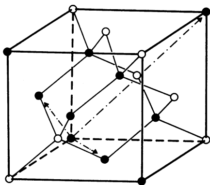
Fig. 8. Microscopically ordered structure produced by annealing of strained germanium-silicon layers. Symbols: (○) silicon atoms; (●) germanium atoms.
