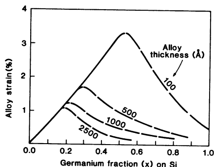
Fig. 5 (left). Tabulation of strain in \text{Ge}_x\text{Si}_{1-x}/\text{Si} films of various thickness and concentration. Fig. 6 (right). Tabulation of critical thickness up to which defect-free germanium-silicon strained-layer epitaxy in \text{Ge}_x\text{Si}_{1-x} layers can be maintained on silicon and germanium substrates. Symbols: (▲) alloys grown on germanium substrates; (●) alloys grown on silicon substrates.
