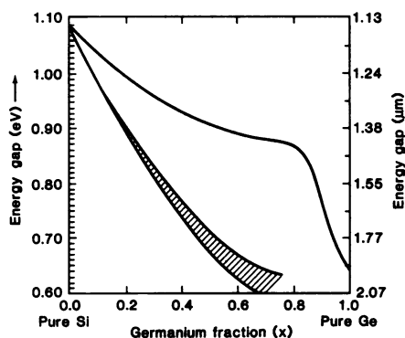
Fig. 2. Energy bandgap for Ge_xSi_{1-x} semiconductor layers. Curves are calculated for unstrained material (upper) and strained-layer epitaxy (lower) on silicon substrates.
