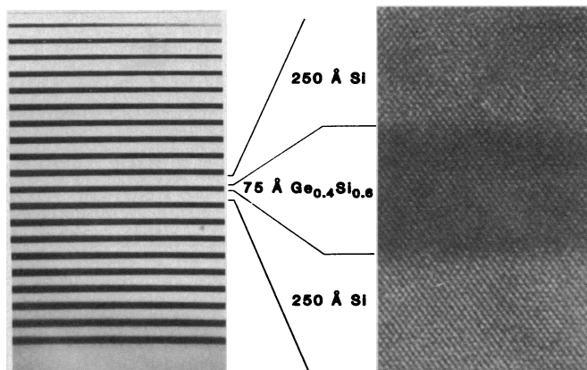
Fig. 7. Cross-sectional TEM micrographs of \text{Ge}_x\text{Si}_{1-x}/\text{Si} strained-layer superlattice (20-period). Enlarged image at right resolves individual atomic rows. [Microscopy by R. Hull and J. M. Gibson]
