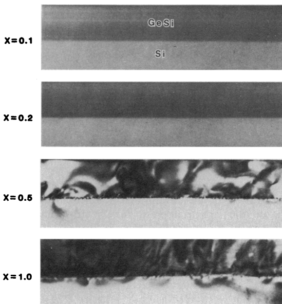
Fig. 4. Cross-sectional TEM micrographs of four \text{Ge}_x\text{Si}_{1-x} layers on silicon substrates. The absence of dislocations in x = 0.1 and 0.2 layers is indicative of strained-layer epitaxy.
