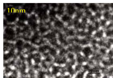
Figure 1 TEM of nanoporous Si
