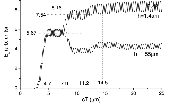
Fig. 2: Amplitude of the electric field varying with the sampling time. The curves labeled by h = 1.4 \mu\text{m} and h = 1.55 \mu\text{m} correspond to the sample with the corresponding slit depth.
