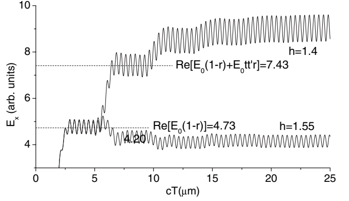
Fig. 5: Sampling time dependence of the electric fields.
