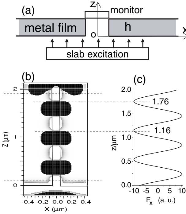
Fig. 1: (a) Sketch of the subwavelength metal slit illuminated by light wave from below. An ideal monitor is set on the slit exit. (b) The pattern of the magnetic field around the slit obtained by FDTD simulation. (c) The x -component of the electric-field distribution in the slit.
