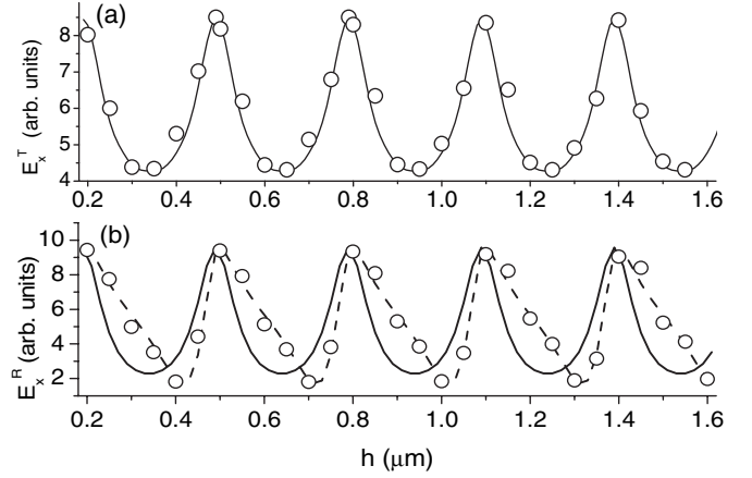
Fig. 3: Dependence of the total electric fields on the film thickness, (a) for transmission light field and (b) for light field just before the illuminated surface. The open circles represent the FDTD simulation results and the solid curve is calculated according to the multi-reflection theory in the PDS model. The dashed line is the corrected calculation result by introducing a phase shift.
