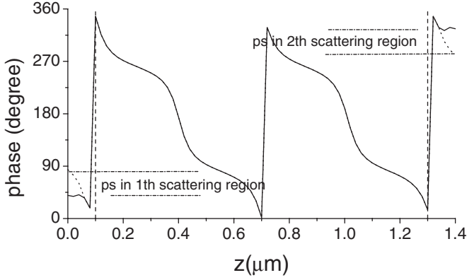
Fig. 4: Simulated phase distributions in the slit of h = 1.4 \mu\text{m} .
