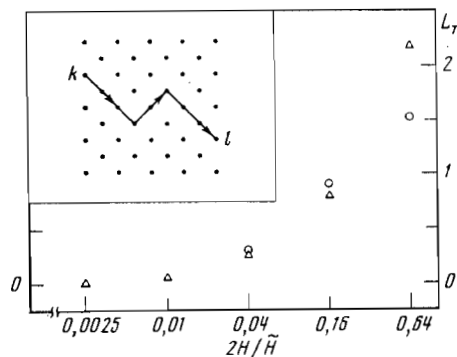
FIG. 8. Results of a calculation of the transparency of the square lattice shown in the inset. \circ —Reference 16; \Delta —Present study.
