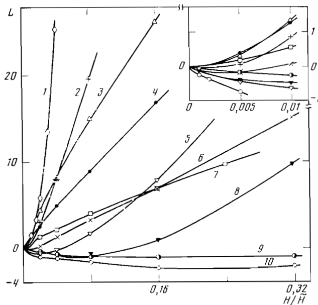
FIG. 7. The quantity L_T + \langle \ln |J(H)/J(0)|^2 \rangle as a function of the dimensionless magnetic field H/\bar{H} for the three-dimensional case and various values of A and x : 1— x=0 ; 2— A=8 , x=0.001 ; 3— A=2 , x=0.5 ; 4— A=20 , x=0.01 ; 5— A=-8 , x=0.01 ; 6— A=-1 , x=0.1 ; 7— A=20 , x=0.1 ; 8— A=-8 , x=0.02 ; 9— A=8 , x=0.1 ; 10— A=-1 , x=0.5 . Shown separately in the inset is the region of very weak fields, H < 0.01 \bar{H} .
