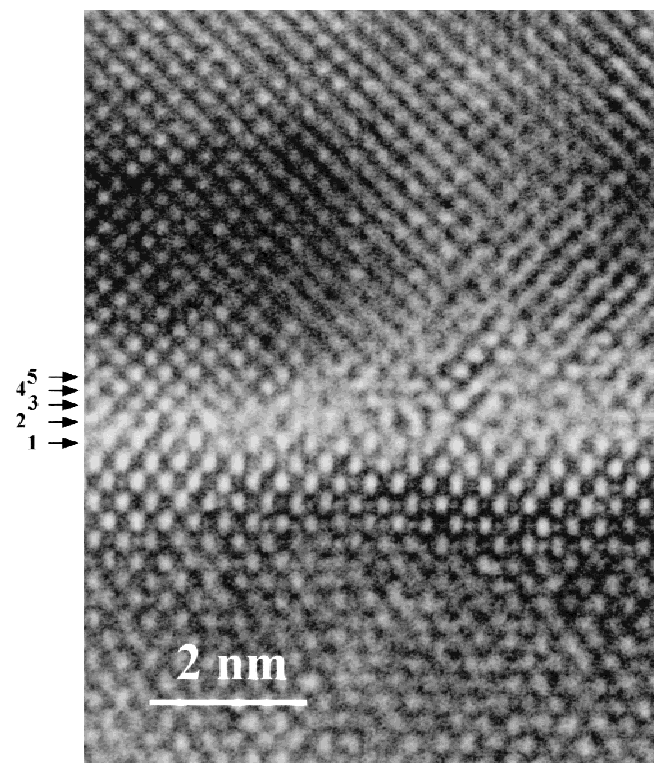
FIG. 4. Enlarged HRTEM image of region B in Fig. 1, showing the sharp interface between the STO thin film and the Si substrate that is noted by the arrowhead numbered as “2”.
