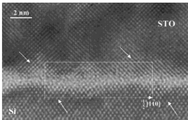
FIG. 3. Enlarged HRTEM image of region A in Fig. 1. Interface dislocation with the Burgers vector of a/2[1\bar{1}0] on the Si side accommodates the misfit of lattice constants between the STO thin film and the Si substrate.
