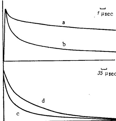
FIG. 1. Relaxation curves of the nonequilibrium conductivity of samples 2 (a, c) and 3 (d), and also of sample 2 in the presence of continuous illumination (b).
