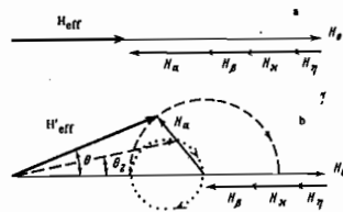
FIG. 8. Diagram of the variation of the effective field H_{\text{eff}} in NMR conditions. a—Away from the resonance; b—in the resonance region of one of the nuclei. The dashed line describes the motion of the tip of the nuclear magnetization vector during adiabatically fast passage through the resonance. The dotted line shows the same for slow passage, when the stationary state is established for each value of \omega .
