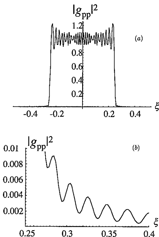
Figure 7. (a) Post-paraxial intensity (36) of the Talbot image of a slit of a Ronchi grating with \epsilon = 0.001\,246 ; this corresponds, for example, to the Talbot plane \zeta = 1 of a grating with a = 0.508 mm (50 lines \text{in}^{-1} ), illuminated by light with \lambda = 632.8 nm. (b) Magnification of (a) showing weak fringes on the dark side of the slit.
