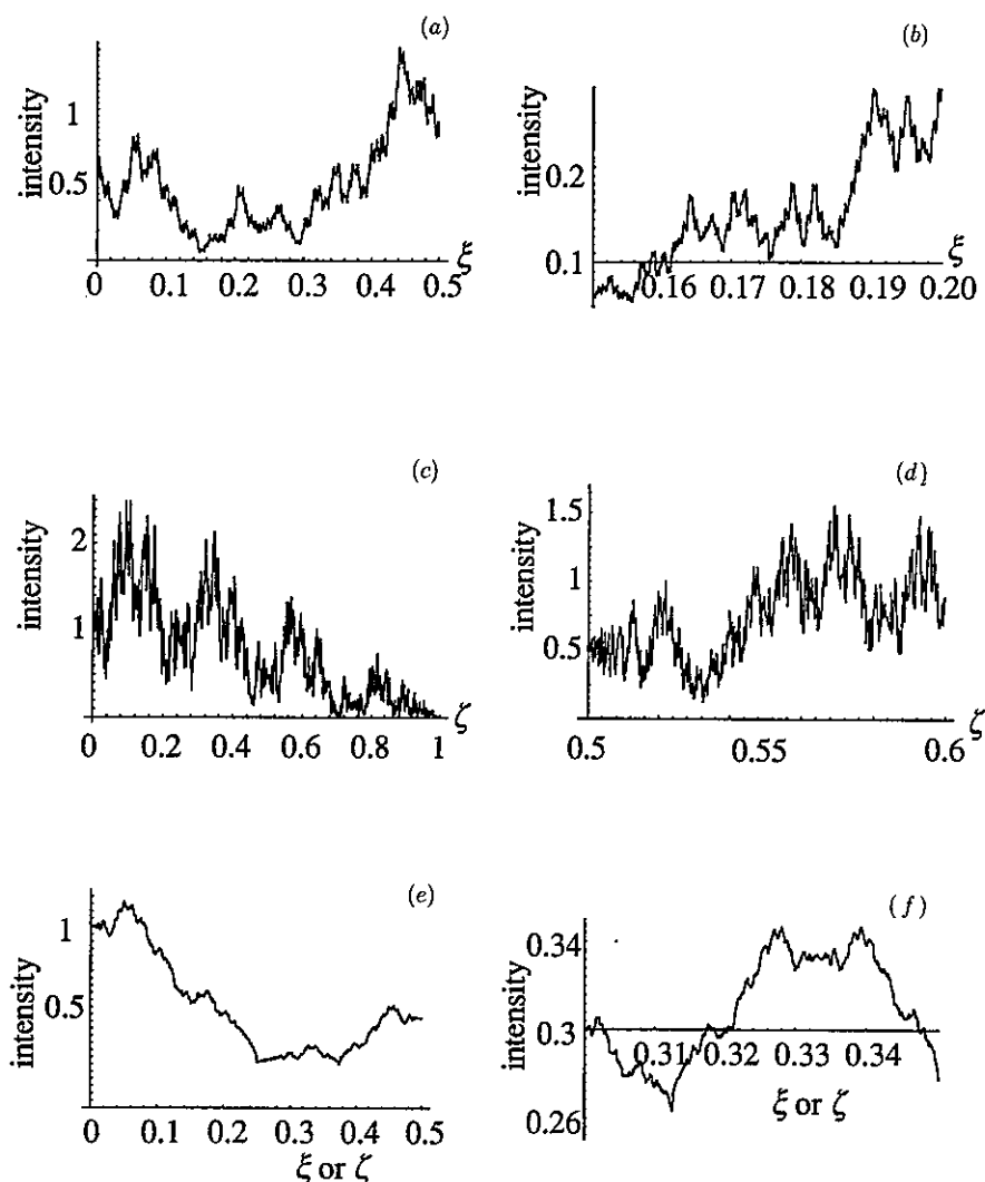
Figure 4. Talbot fractals and their magnifications: (a) transverse fractal, with dimension D_\xi = \frac{3}{2} , in the plane \zeta = \zeta_G ; (b) magnification of (a); (c) longitudinal Talbot fractal, with dimension D_\zeta = \frac{7}{4} , in the plane \xi = 0 ; (d) magnification of (c); (e) diagonal Talbot fractal, with dimension D_d = \frac{5}{4} , in the plane \xi = \zeta ; (f) magnification of (e).
