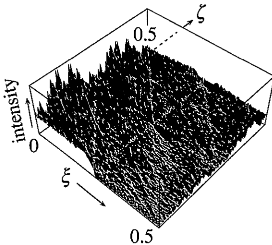
Figure 5. The 'mountains of Talbot', displaying the paraxial light intensity behind a Ronchi grating as a surface with fractal dimension \frac{11}{4} .
