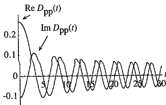
Figure 6. Post-paraxial generalization (34) of the \delta function, describing the blurring of the Talbot images.
