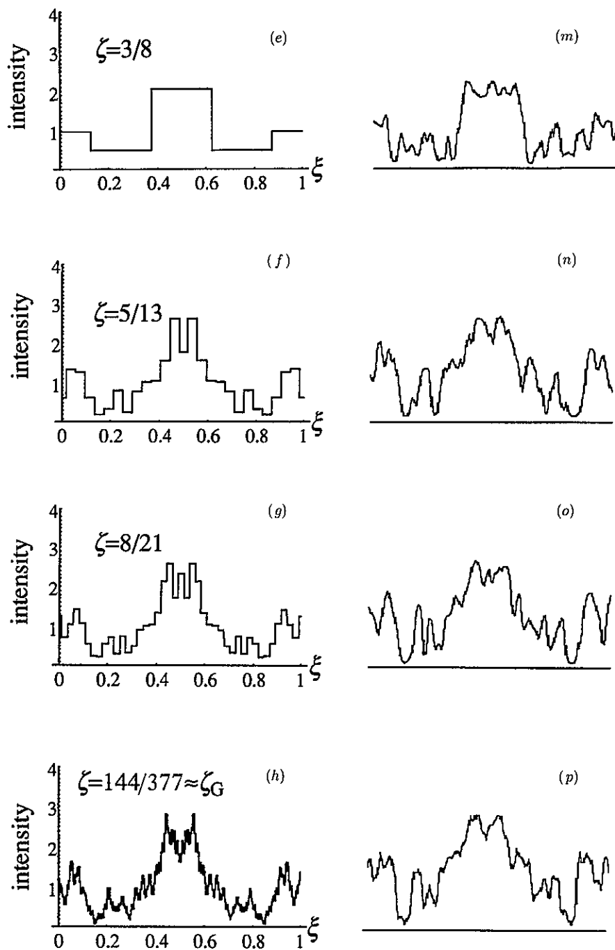
Figure 2. (a)–(h) Calculated intensities in a unit cell, for Talbot planes with \zeta = 1 and \zeta given by the indicated rational approximations to the golden distance \zeta_G = (3 - 5^{1/2})/2 , for the Ronchi grating (2). The transverse Talbot fractal, with dimension D_\xi = \frac{3}{2} , appears in (h). (i)–(p) Observed intensities in Talbot planes corresponding to (a)–(h), with a Ronchi grating with a = 0.508 mm (50 lines \text{in}^{-1} ), of which 100 lines were illuminated by a laser with \lambda = 632.8 nm.
