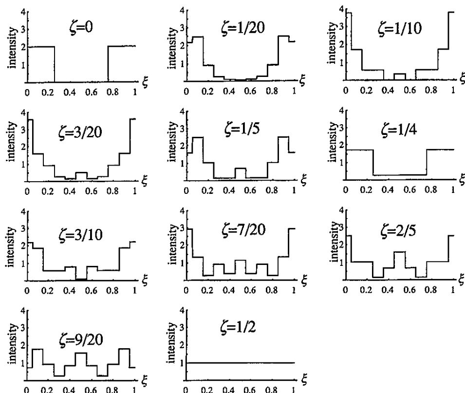
Figure 1. Intensities in one unit cell of the Talbot planes \zeta = n/20 ( 0 \leq n \leq 10 ), for the Ronchi grating (2).
