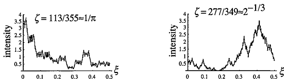
Figure 3. Transverse Talbot intensities, calculated in half-unit cells of planes approximating the distances \zeta = 1/\pi and 2^{-1/3} , for the Ronchi grating (2). Note that 1/\pi - 113/355 = 2.7 \times 10^{-8} , 2^{-1/3} - 277/349 = 4.3 \times 10^{-6} .
