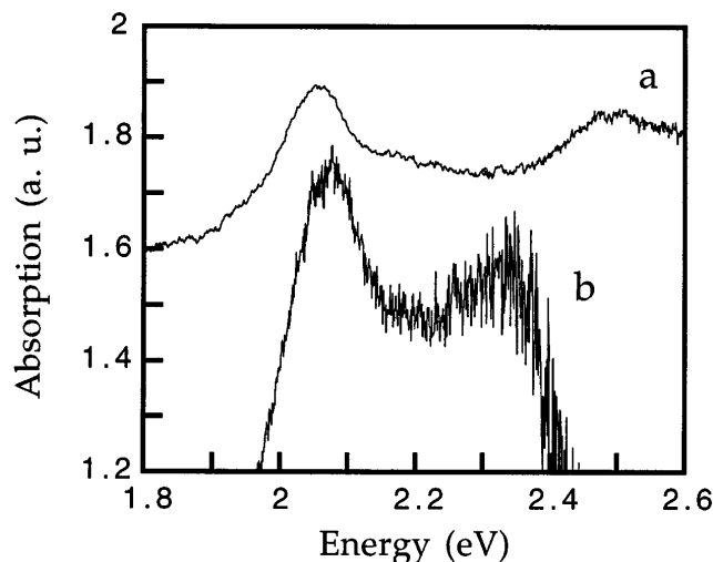
FIG. 4. Absorption spectra at 25 K of (a) 2H- \text{WS}_2 bulk and (b) \text{WS}_2 nanotubes 150–200 Å in diameter and 1500–3000 Å in length, with 1–2 layers.
